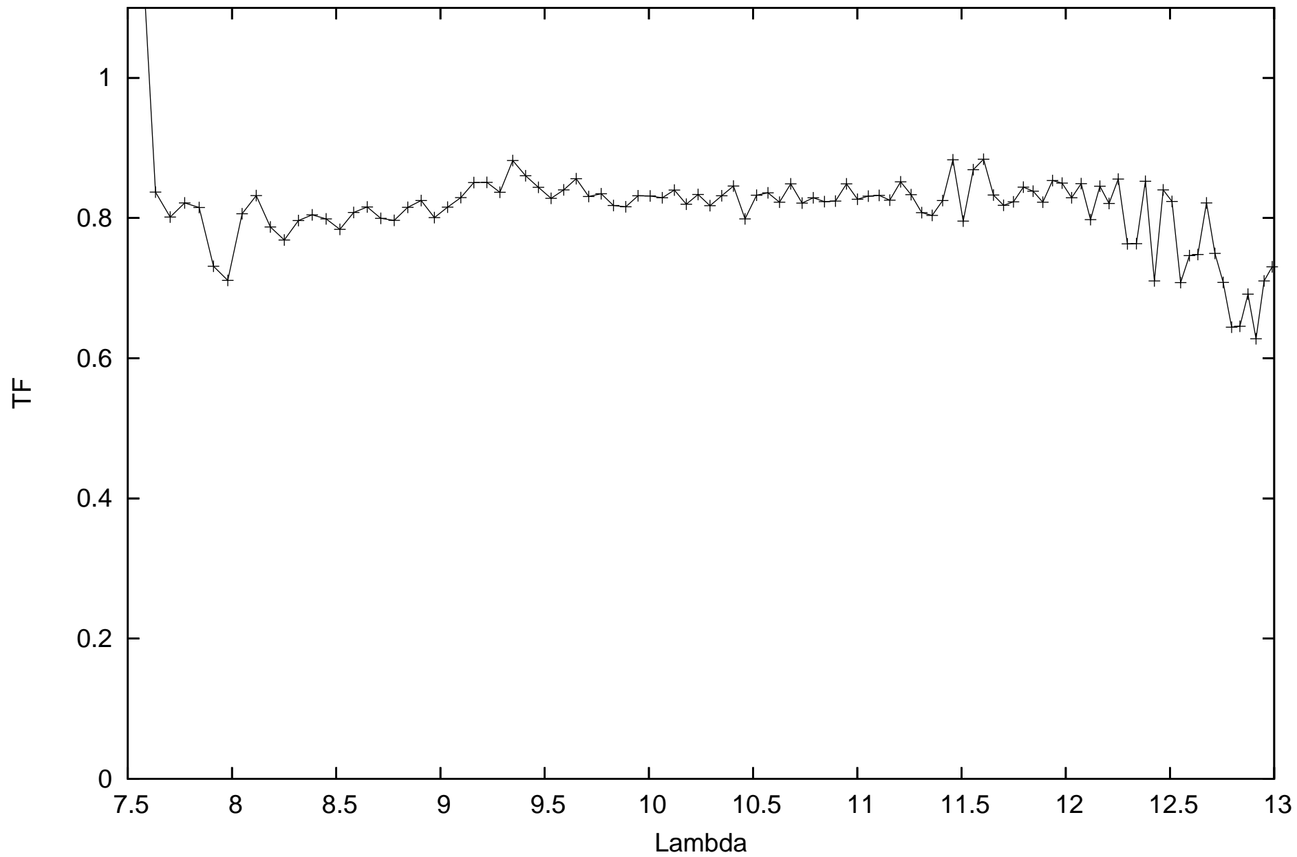
calHD48915_flux-1.39_diam6.09_r.MIDI.2014-01-19T03_27_30.969_B2A1
