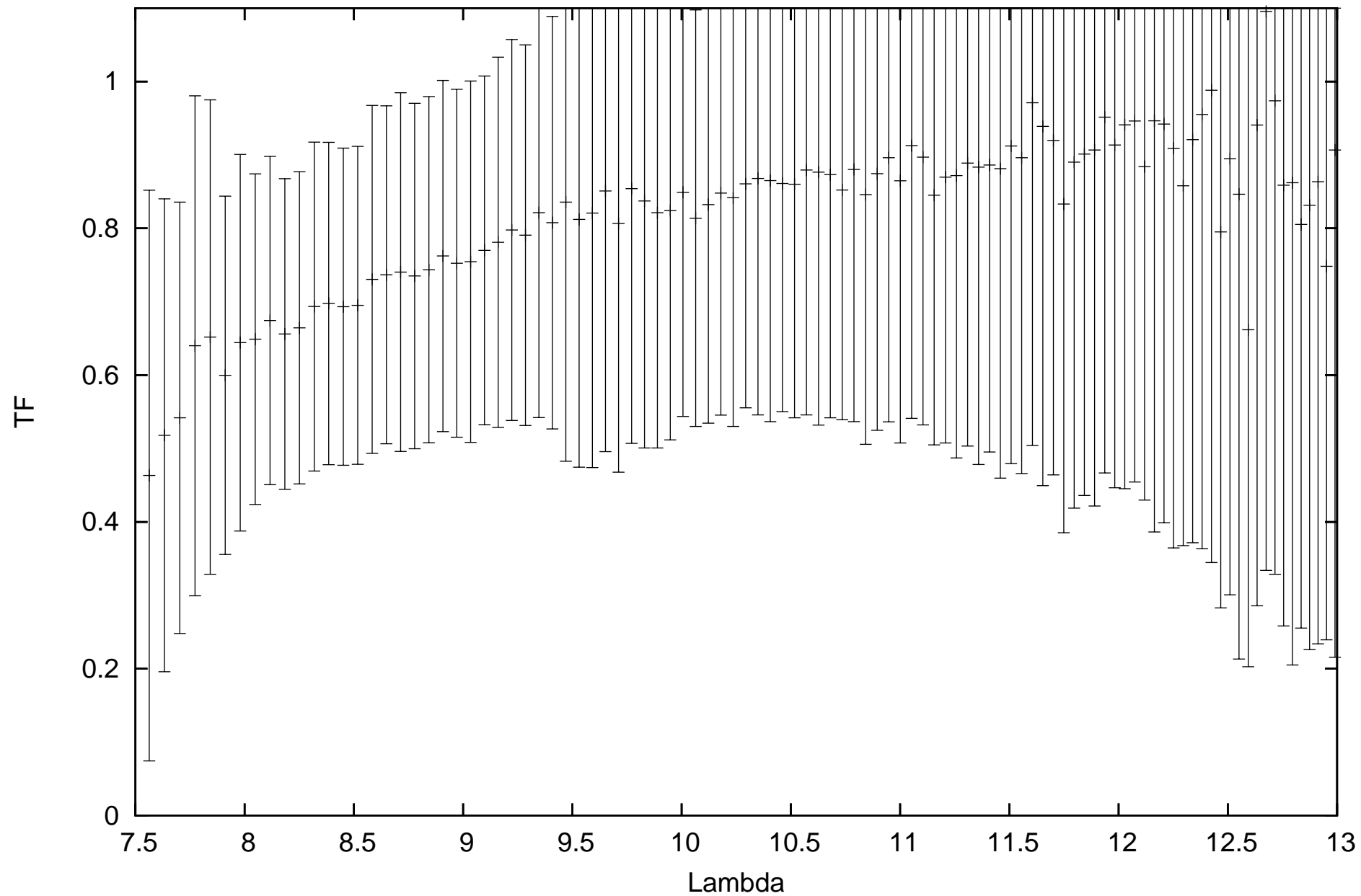
calHD48915_flux-1.39_diam6.09_r.MIDI.2014-01-06T05_54_59.970_D0H0
