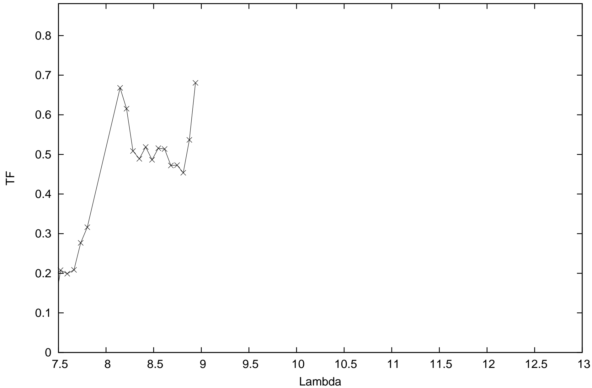
calHD187642_flux0.2_diam3.31_r.MIDI.2014-07-06T06_57_01.000_B2A1
