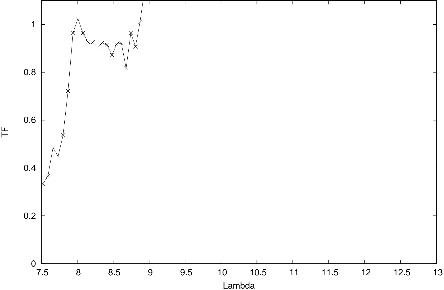
calHD187642_flux0.2_diam3.31_r.MIDI.2014-07-06T06_18_31.000_B2A1
