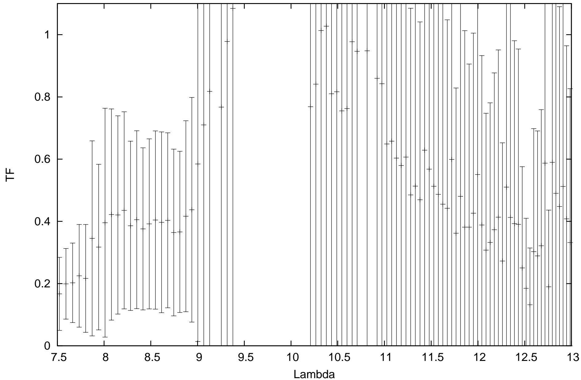
calHD187642_flux0.2_diam3.31_r.MIDI.2014-07-06T05_17_27.000_B2A1
