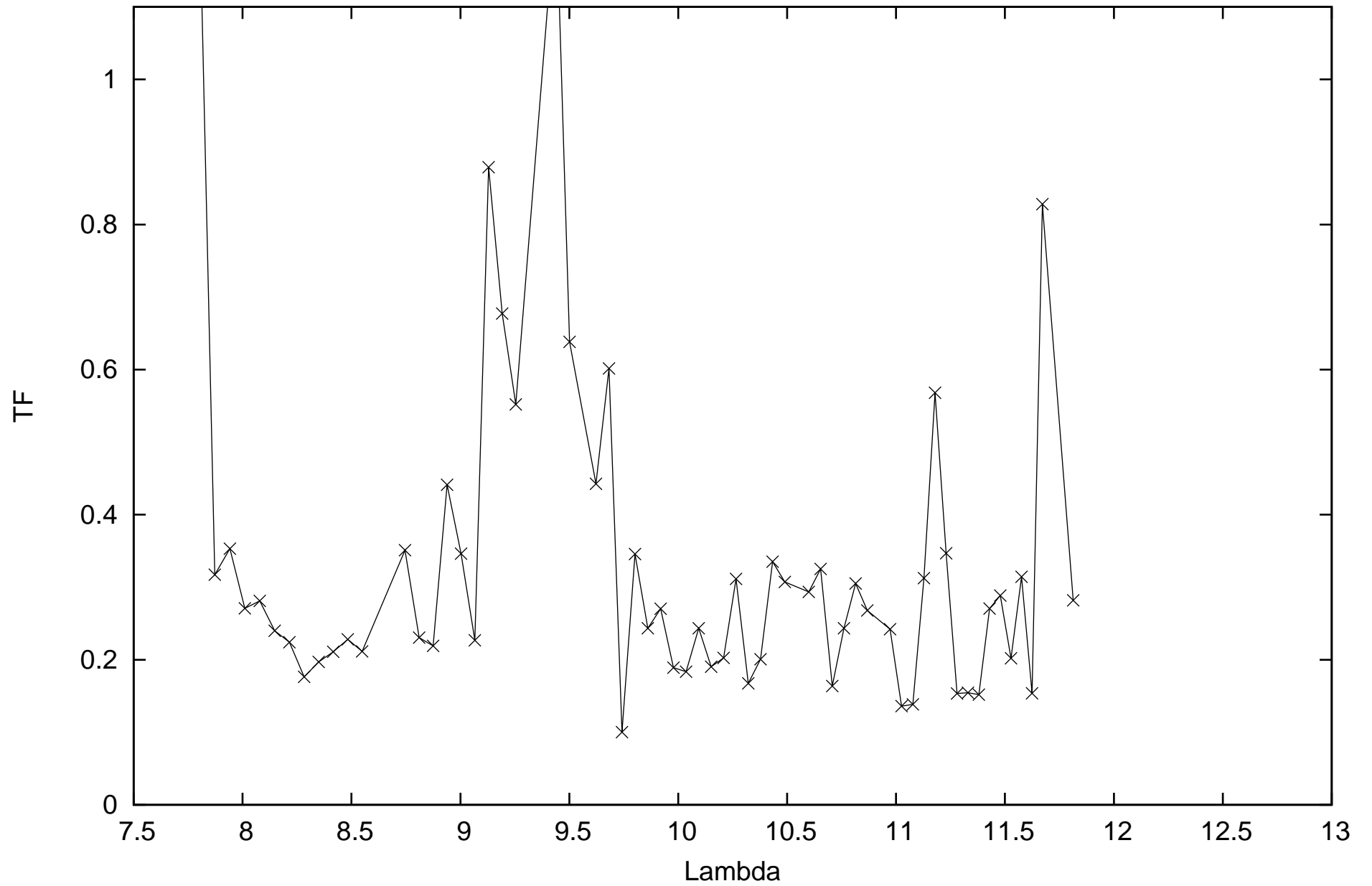
calHD176541_flux0.63_diam3.94_r.MIDI.2014-04-07T08_46_56.000_D011
