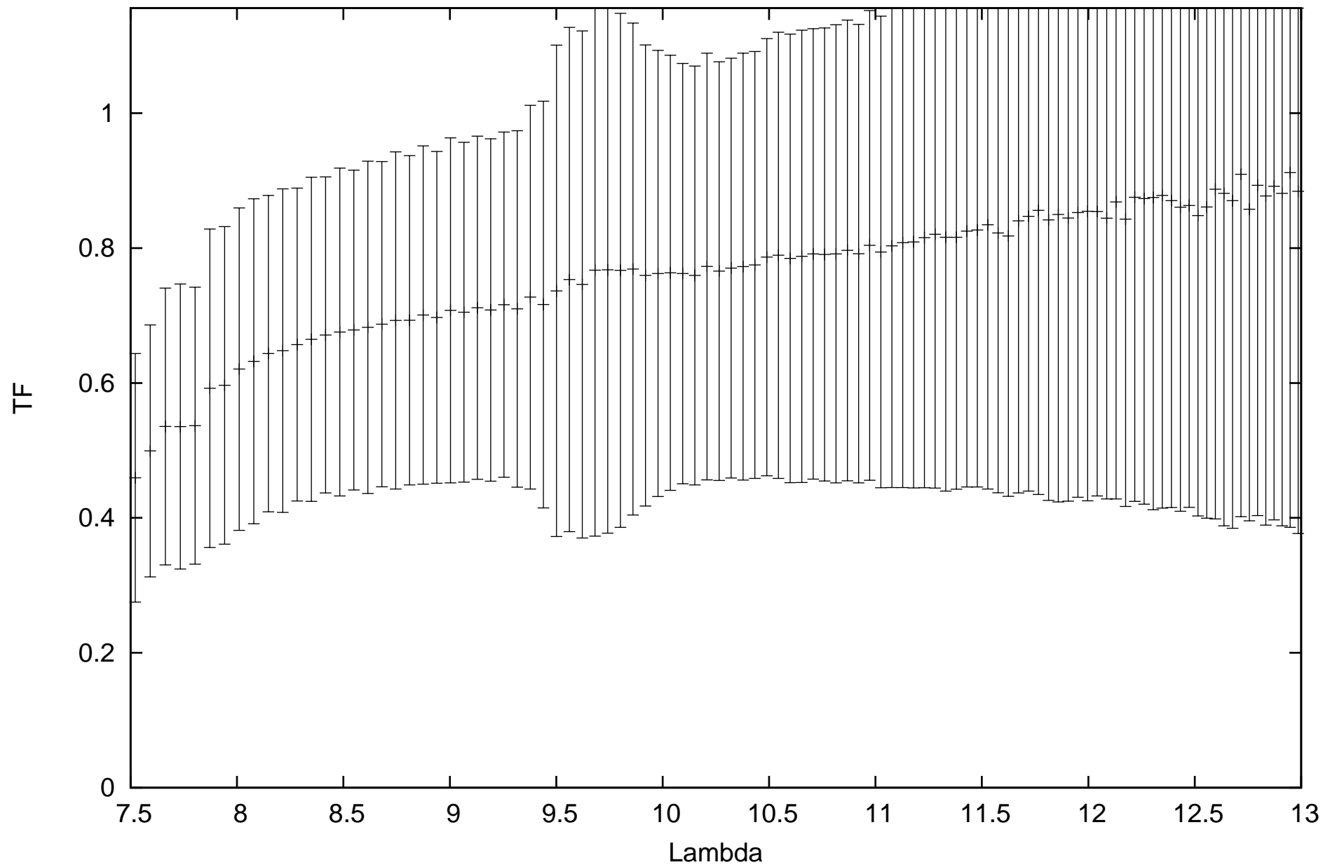
calHD151011_flux1.28_diam2.85_r.MIDI.2014-04-16T09_42_57.000_U3U4
