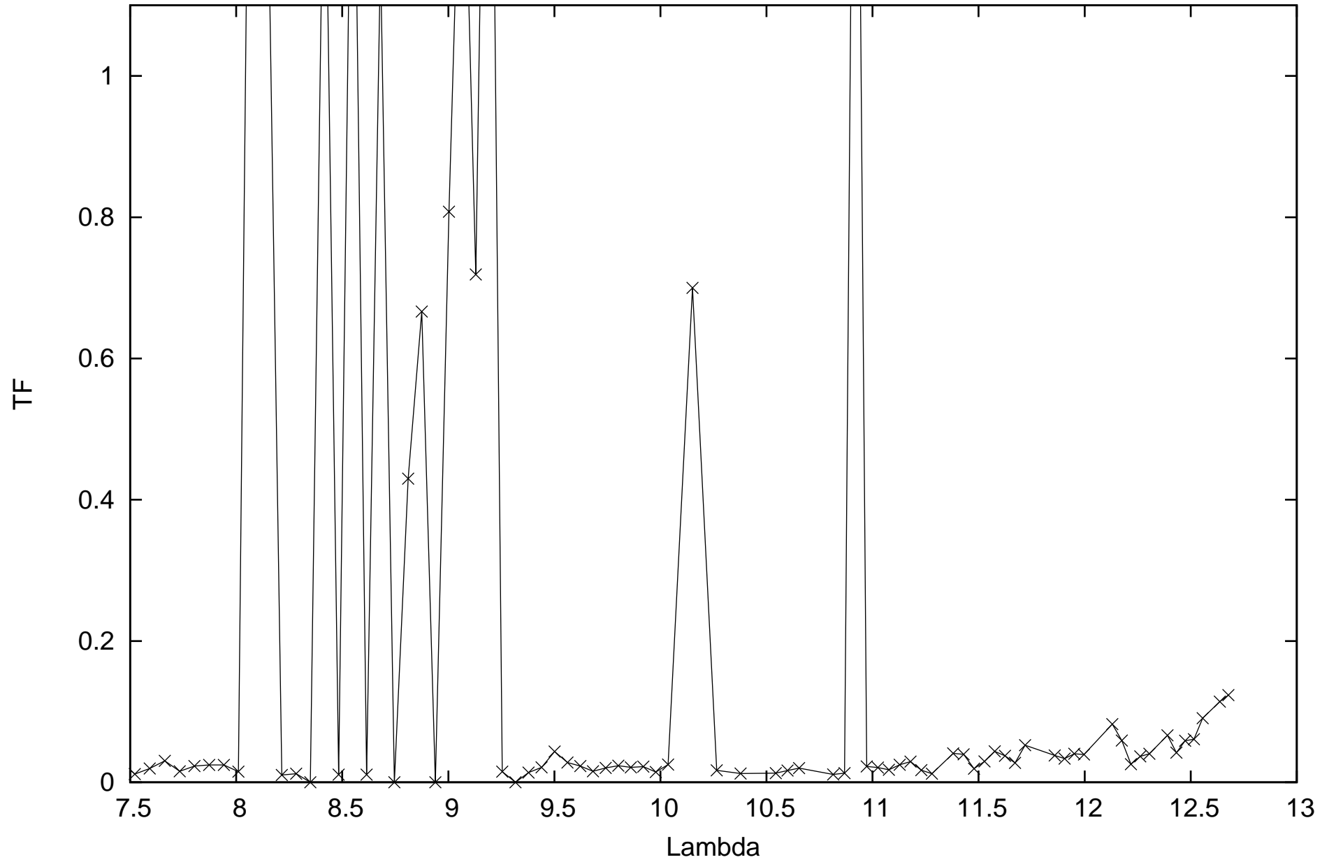
calHD48915_flux-1.39_diam6.09_r.MIDI.2014-12-29T04_13_31.000_C1A1
