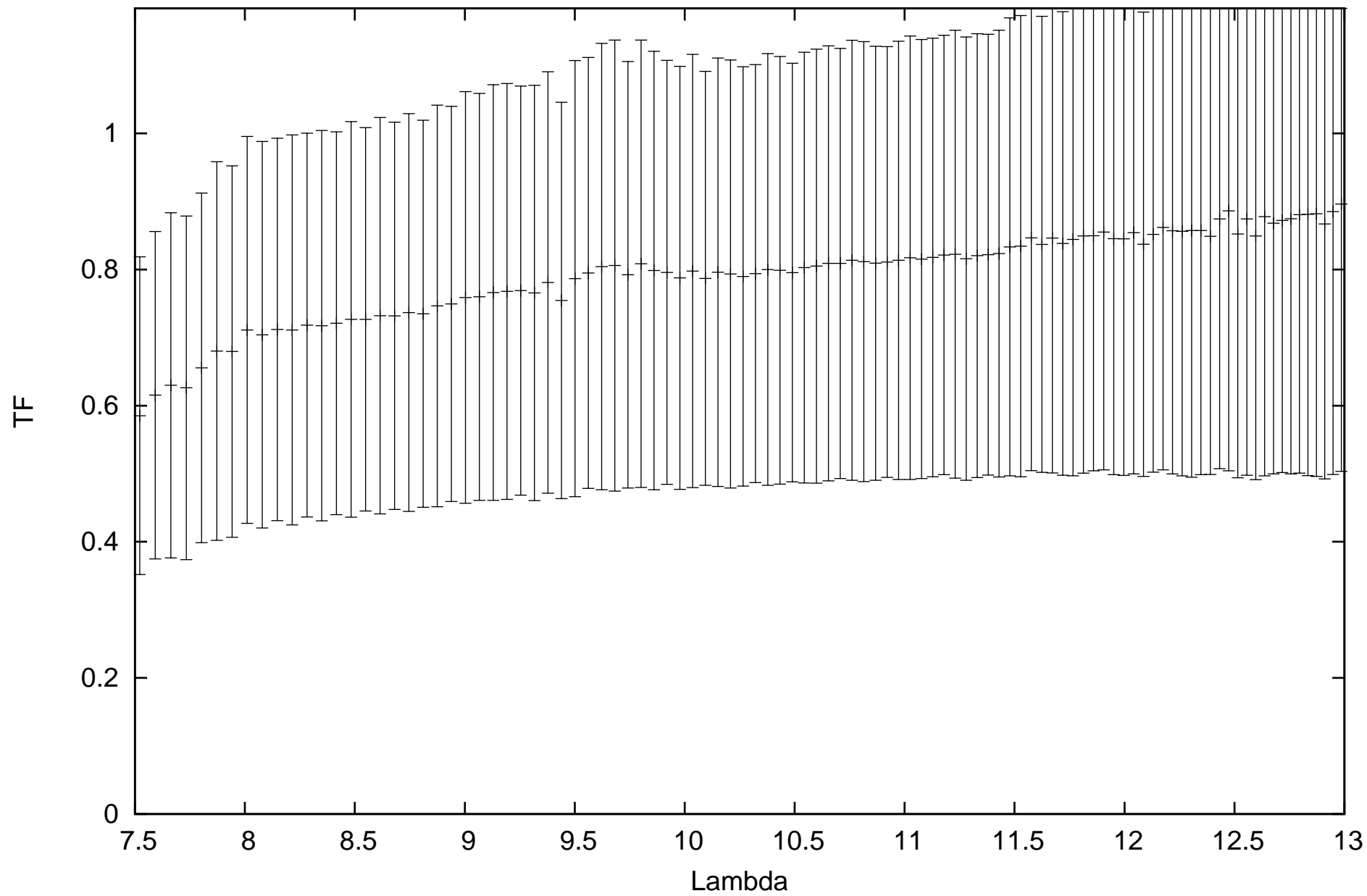
calHIP21421_flux-3.13927_diam20.4_r.MIDI.2014-12-27T02_58_56.000_B2A1
