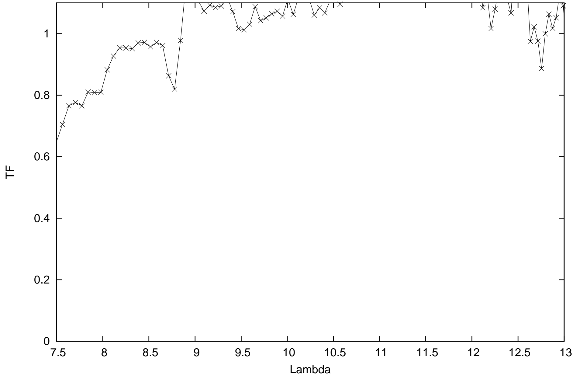
calHD48915_flux-1.39_diam6.09_r.MIDI.2014-12-26T04_15_05.113_D0B2
