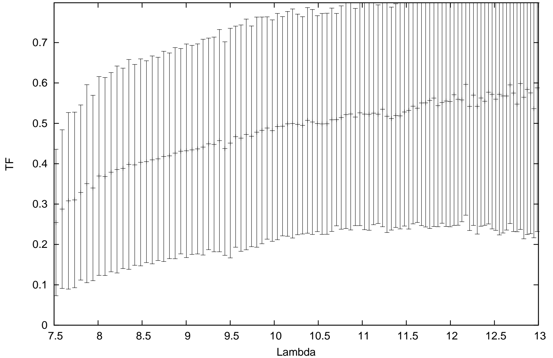
calHD48915_flux-1.39_diam6.09_r.MIDI.2014-12-02T03_48_42.000_G1A1
