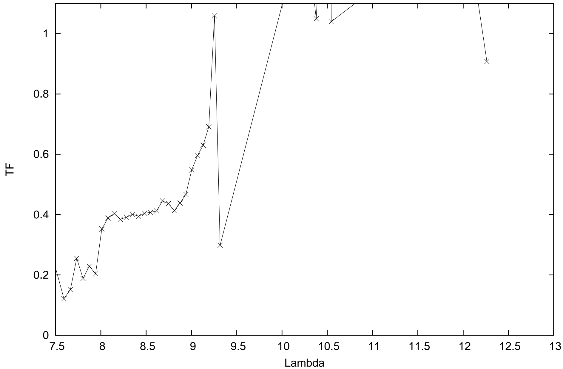
calHIP3419_flux-0.47009_diam5.23_r.MIDI.2014-12-01T05_10_40.000_K0A1
