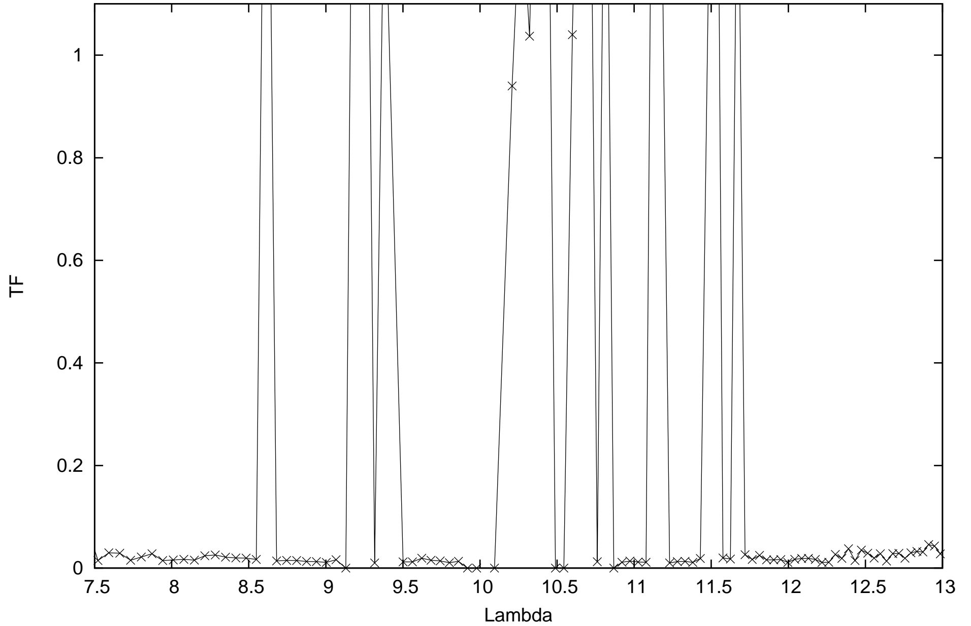
calHD48915_flux-1.39_diam6.09_r.MIDI.2014-10-18T08_54_40.000_G1A1
