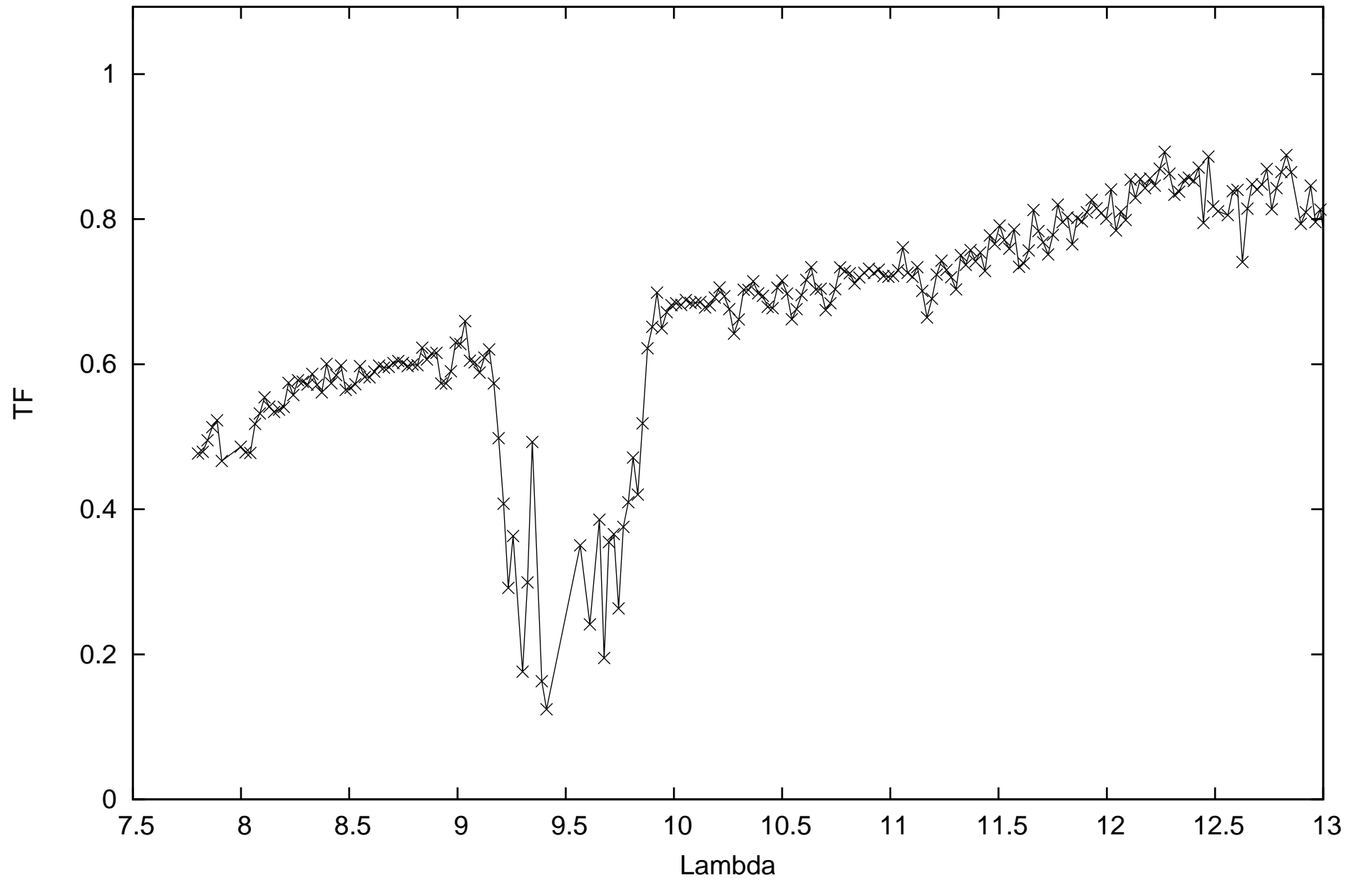
calHD167618_flux-1.82_diam11.66_r.MIDI.2014-10-11T01_19_58.000_C1A1
