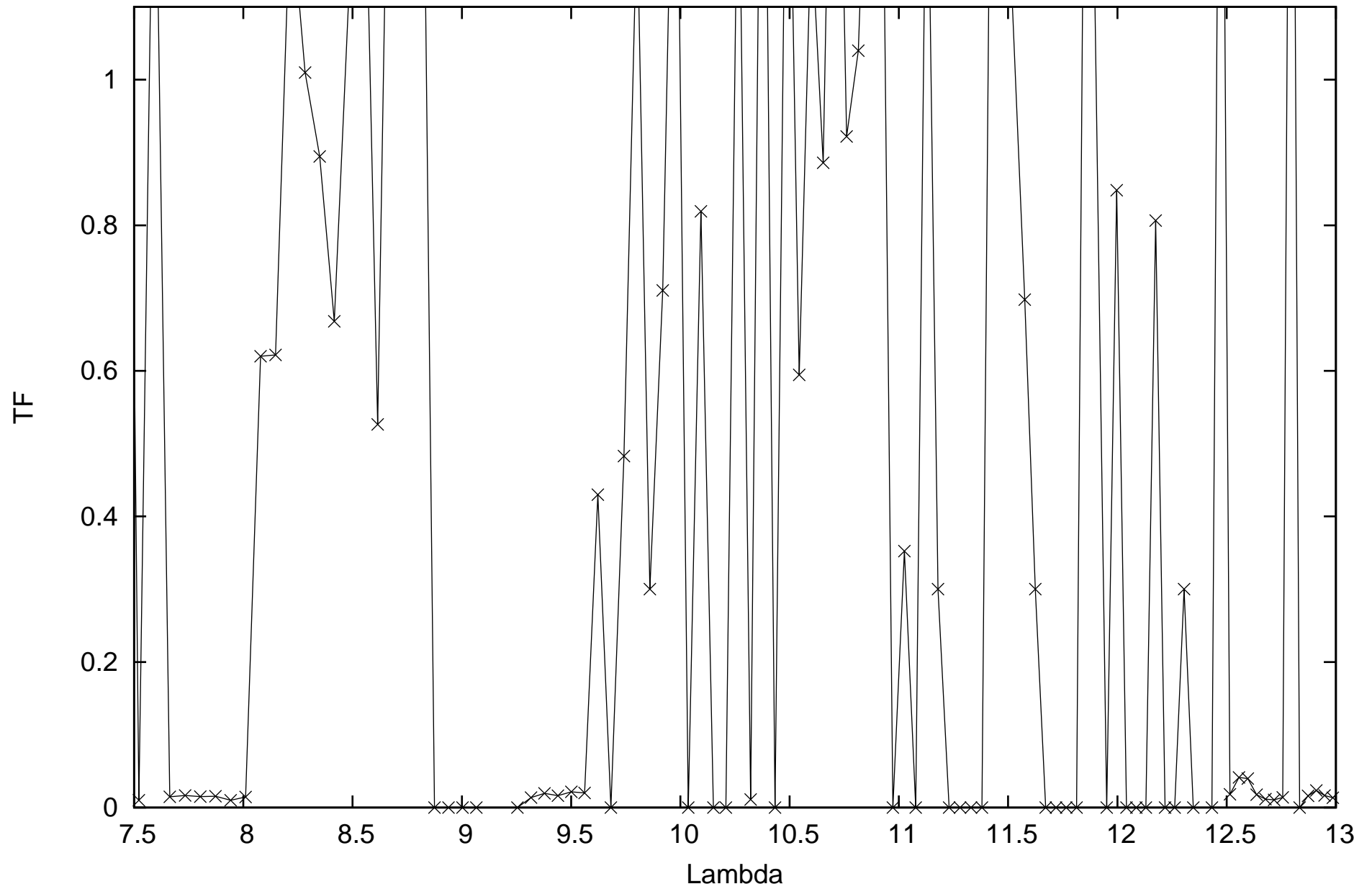
calHIP3419_flux-0.47009_diam5.23_r.MIDI.2014-10-10T02_58_39.000_U2U4
