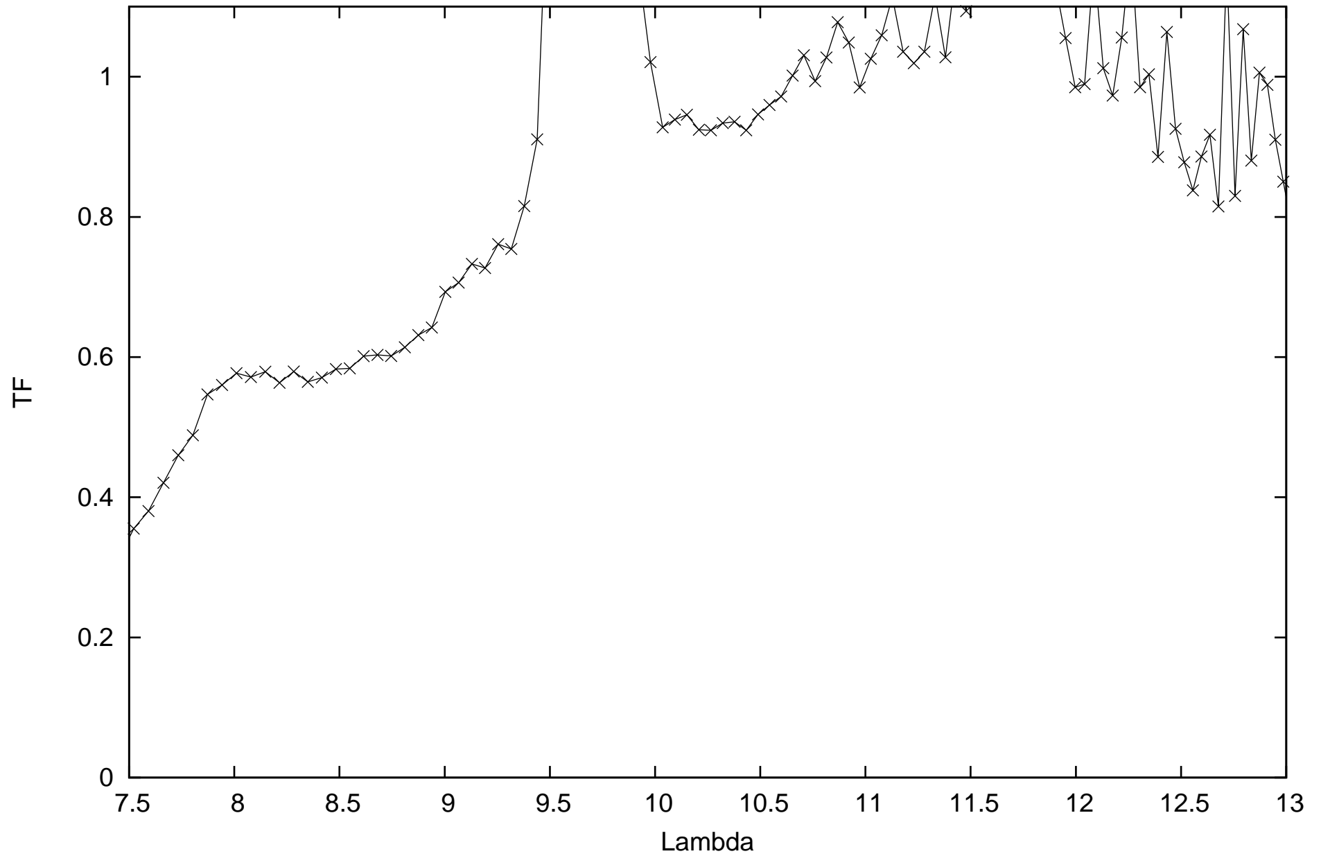
calHIP3419_flux-0.47009_diam5.23_r.MIDI.2014-09-28T02_52_53.000_H0G1
