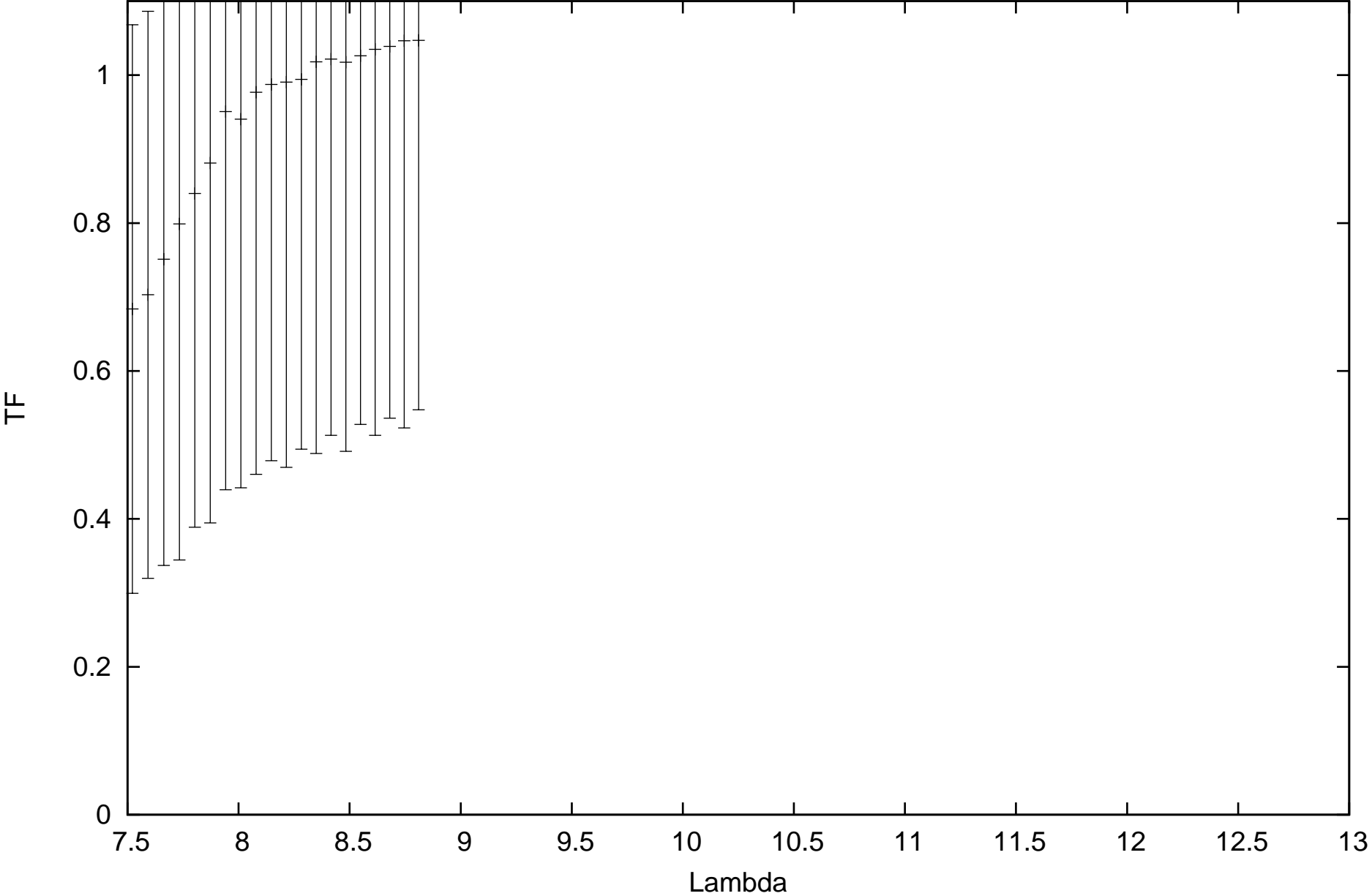
calHD20720_flux-1.53_diam10.14_r.MIDI.2014-09-28T07_23_24.000_D0H0
