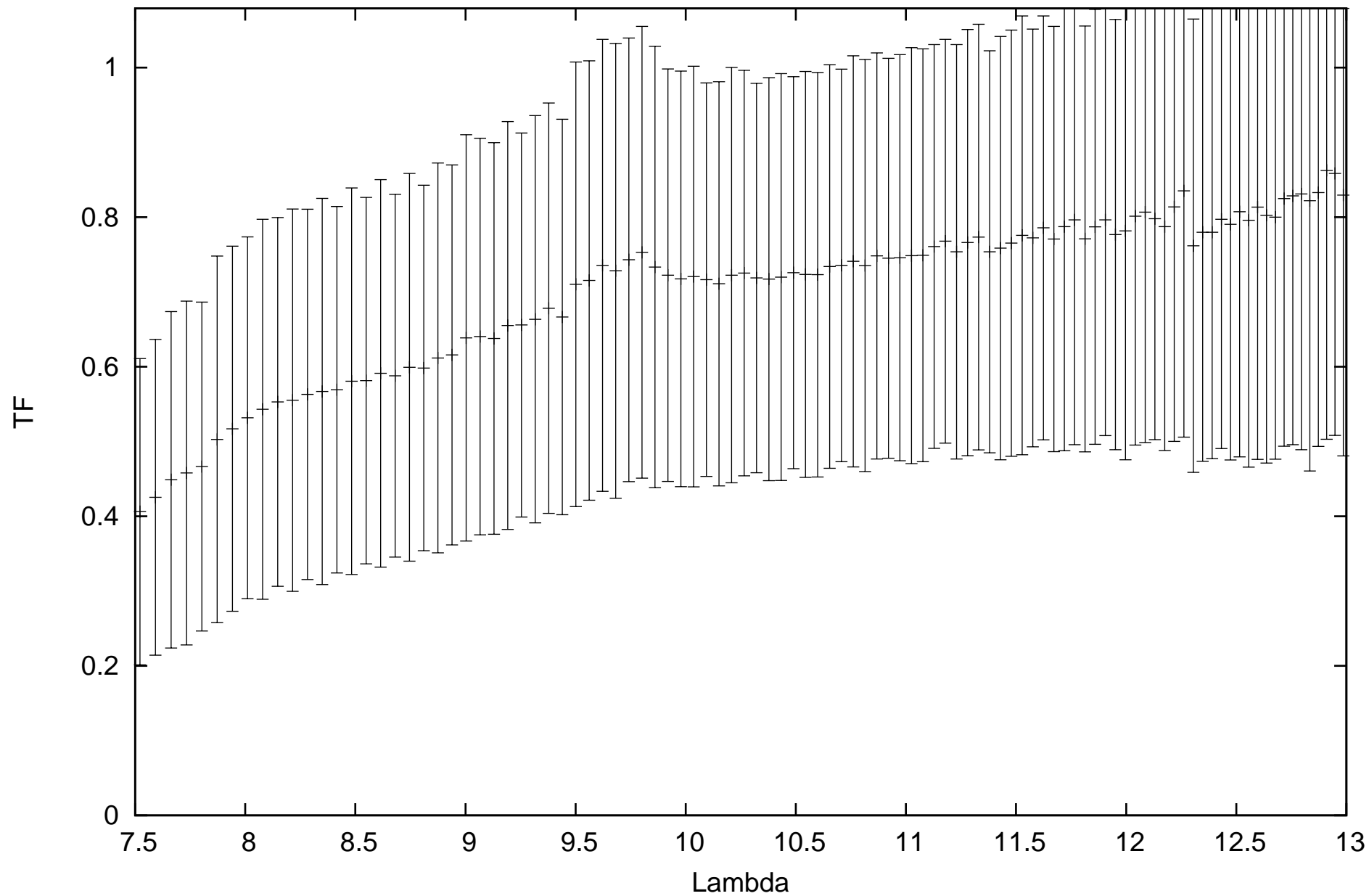
calHD20720_flux-1.53_diam10.14_r.MIDI.2014-09-28T07_09_45.000_D0H0
