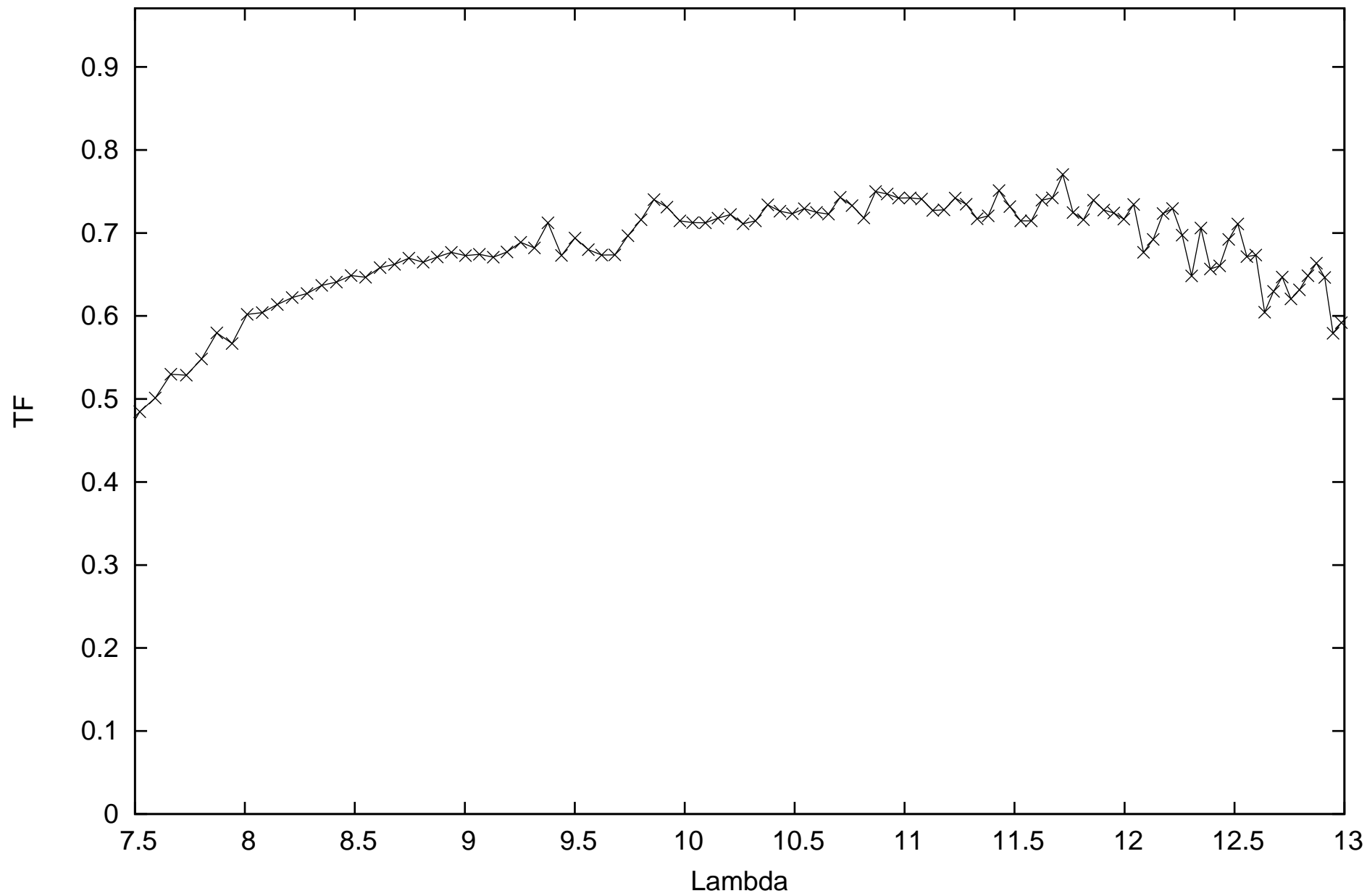
calHIP3419_flux-0.47009_diam5.23_r.MIDI.2014-09-24T03_22_34.000_C1B2
