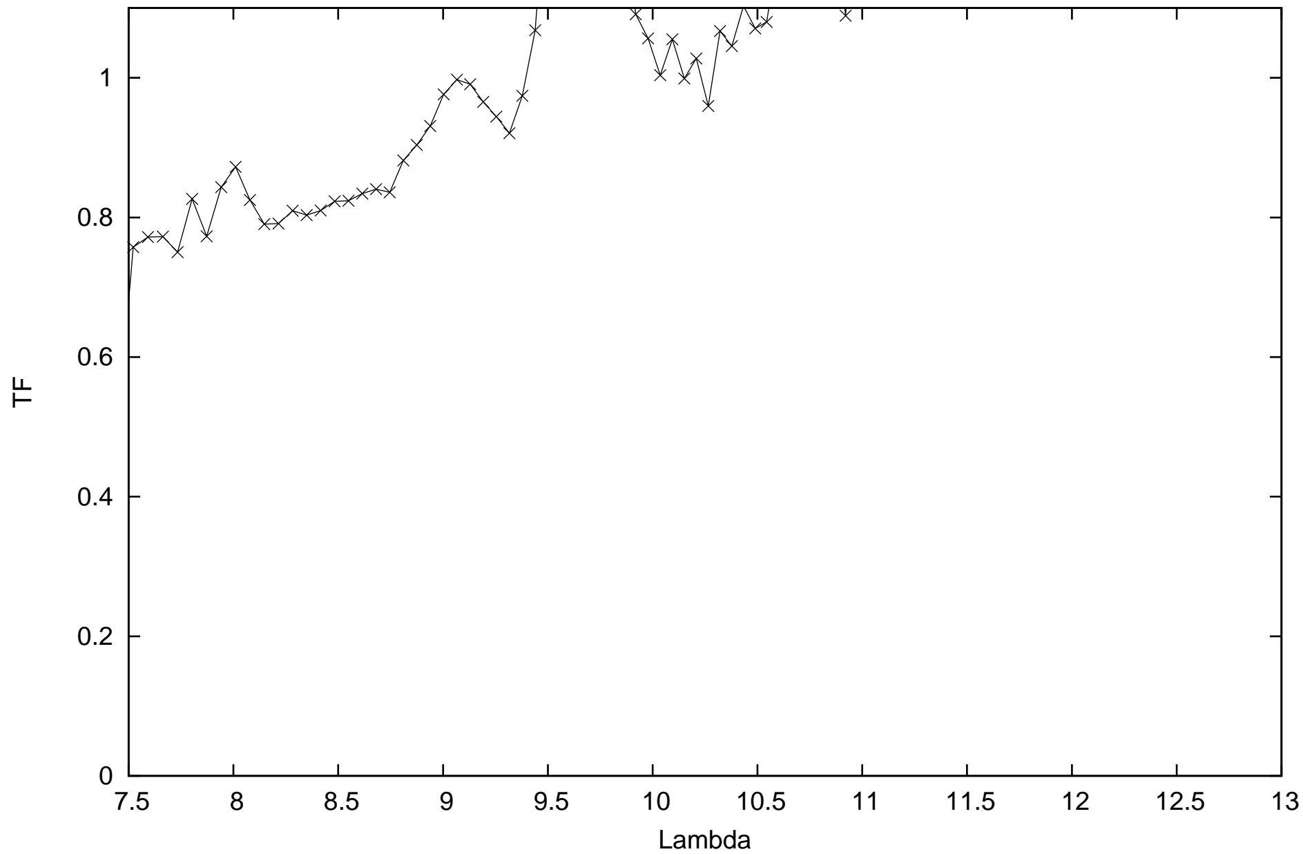
calHIP90496_flux0.238088_diam3.99_r.MIDI.2014-09-07T01_43_20.000_D0C1
