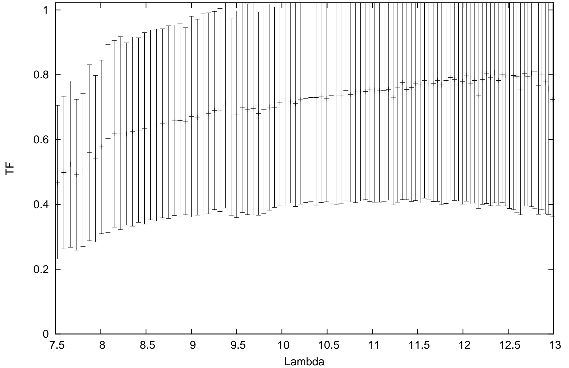
calHIP110997_flux1.58908_diam2.11_r.MIDI.2014-08-09T07_24_54.000_U1U2
