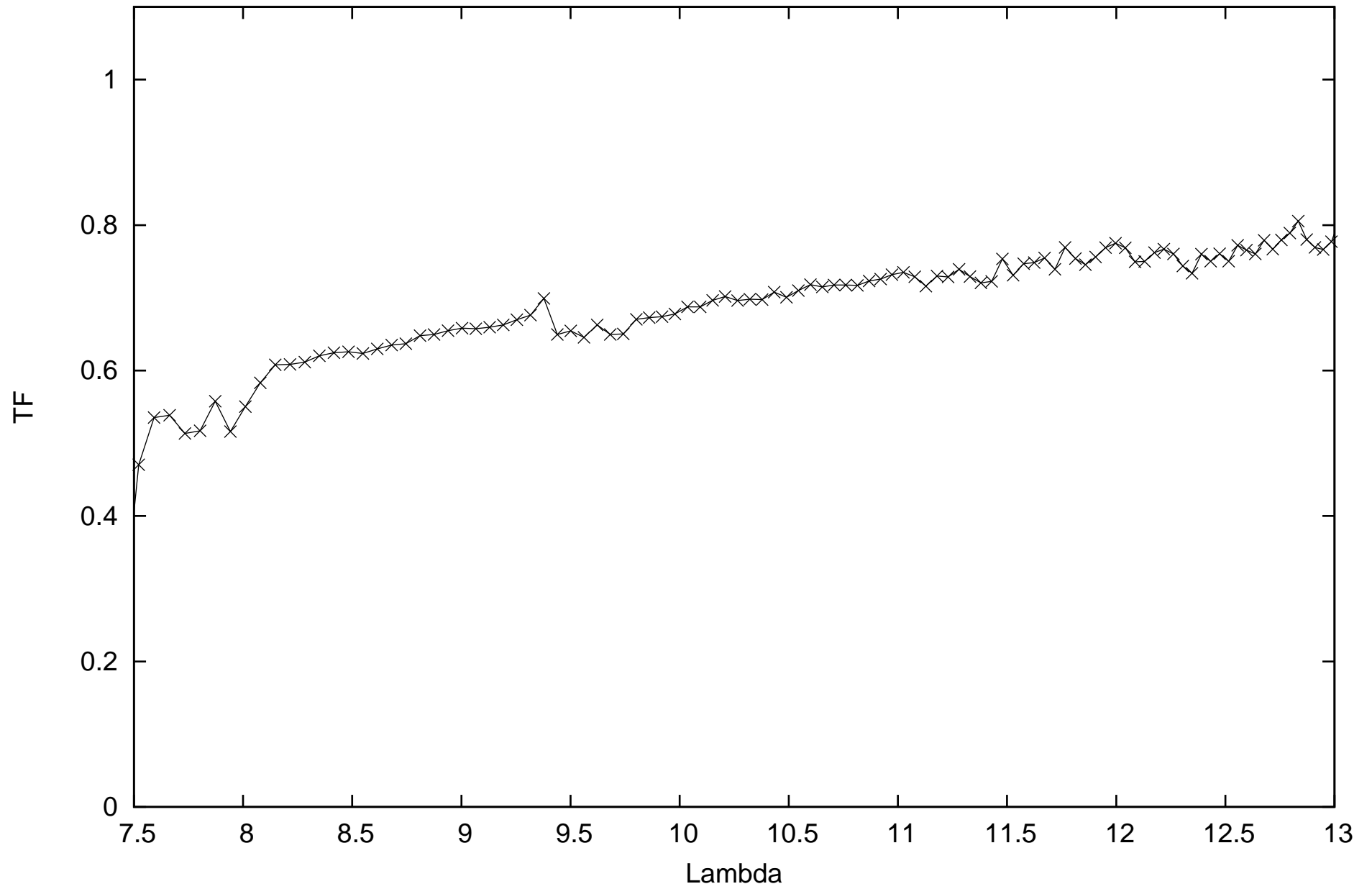
calHD10052_flux1.2_diam3._r.MIDI.2014-08-08T04_27_43.000_U2U4
