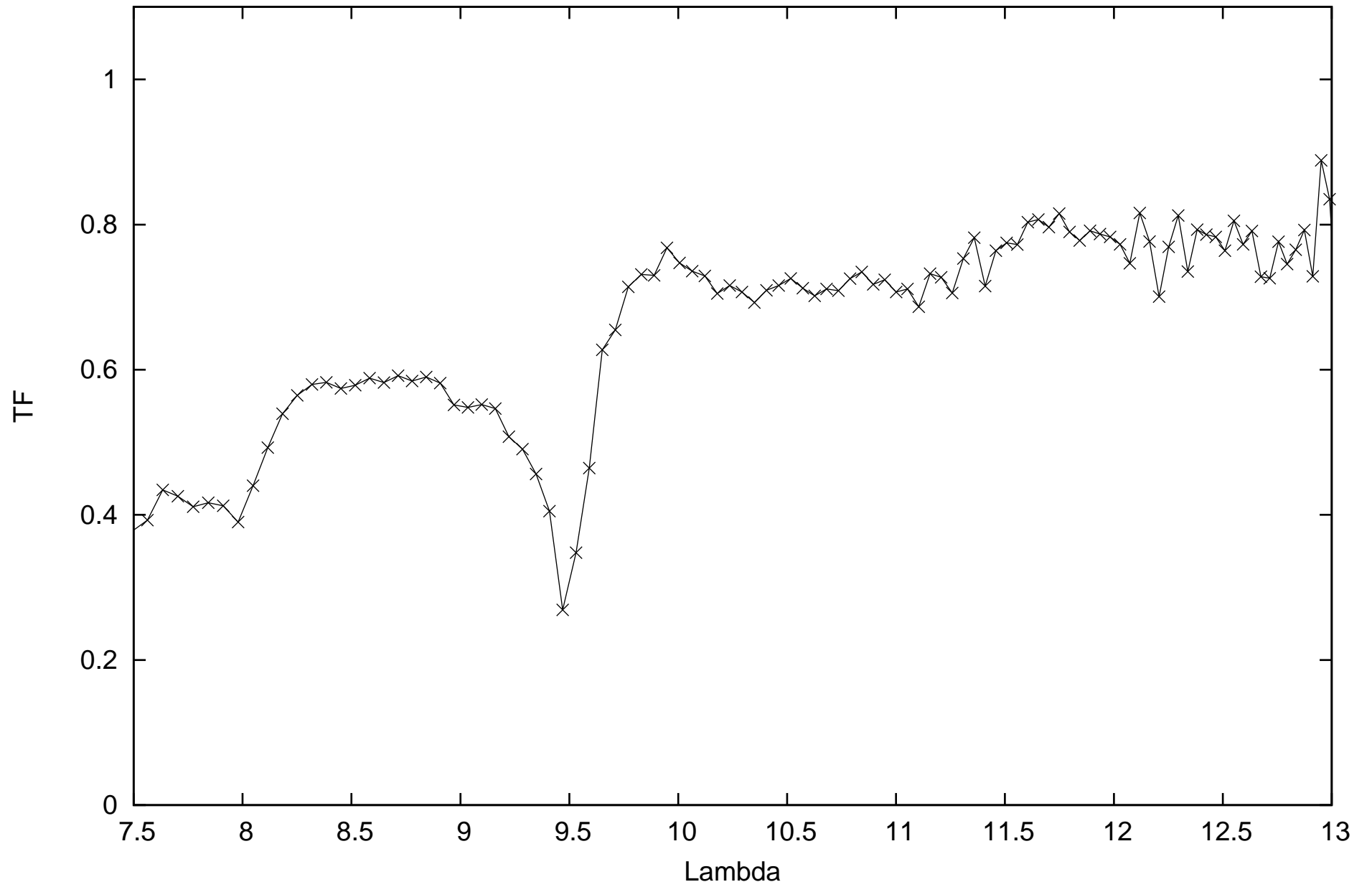
calHIP73714_flux-1.78451_diam11.15_r.MIDI.2014-07-19T00_45_31.113_G1A1
