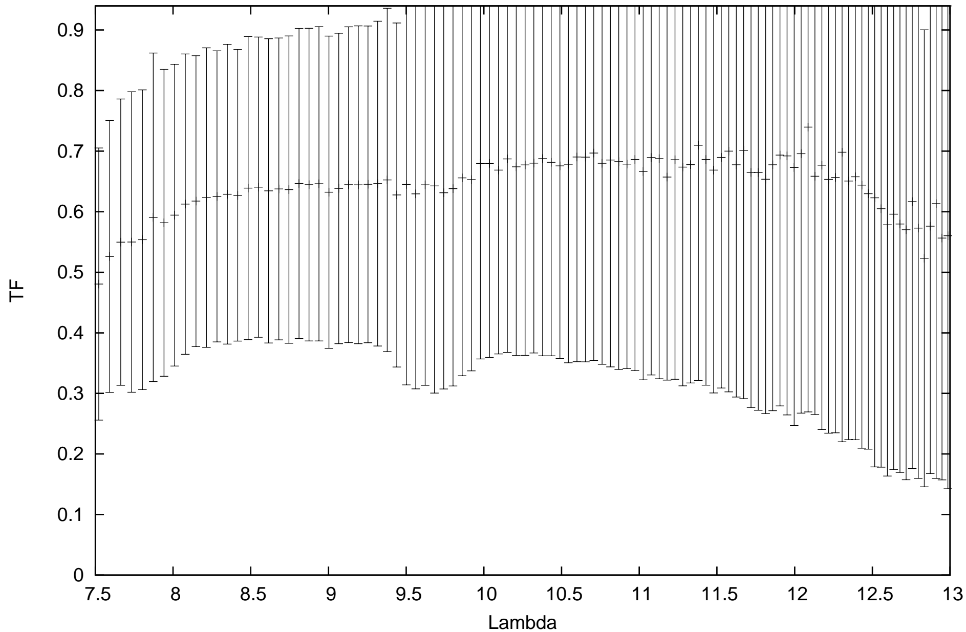
calHIP89931_flux-0.511_diam5.87_r.MIDI.2014-07-16T01_28_49.000_G1A1
