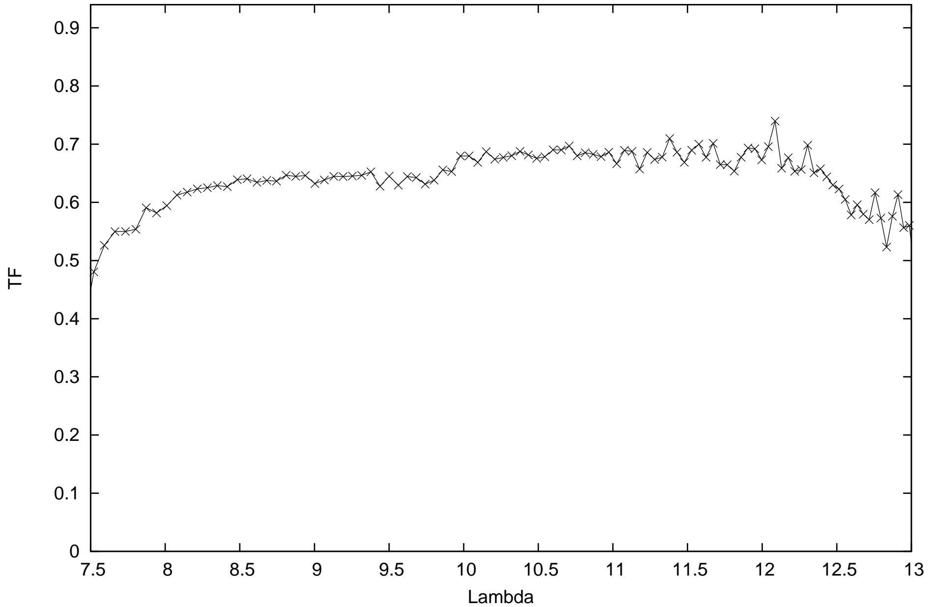
calHIP89931_flux-0.511_diam5.87_r.MIDI.2014-07-16T01_28_49.000_G1A1
