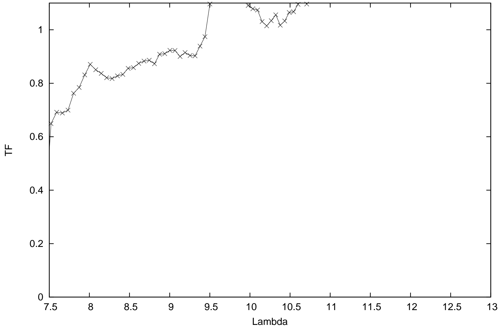
calHIP89931_flux-0.511_diam5.87_r.MIDI.2014-07-14T00_54_19.000_G1A1
