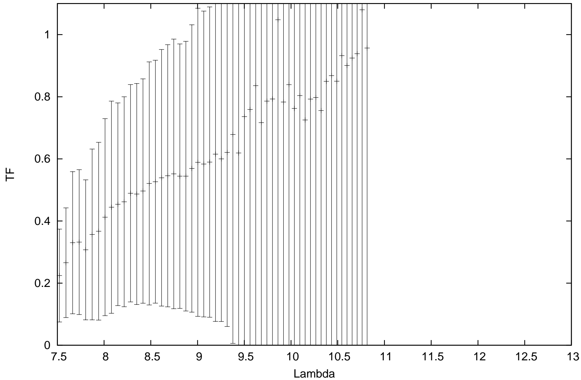
calHIP82363_flux-0.3207_diam5.52_r.MIDI.2014-06-30T03_05_15.000_J3G1
