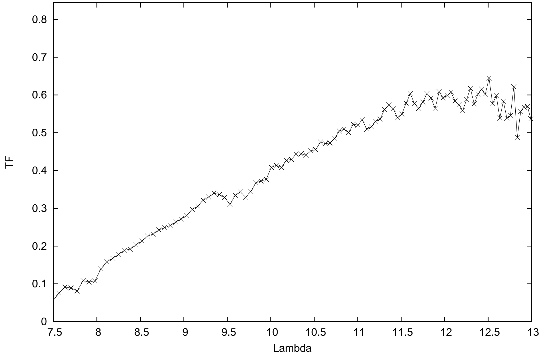
calHD167618_flux-1.82_diam11.66_r.MIDI.2014-06-30T02_40_08.113_J3G1
