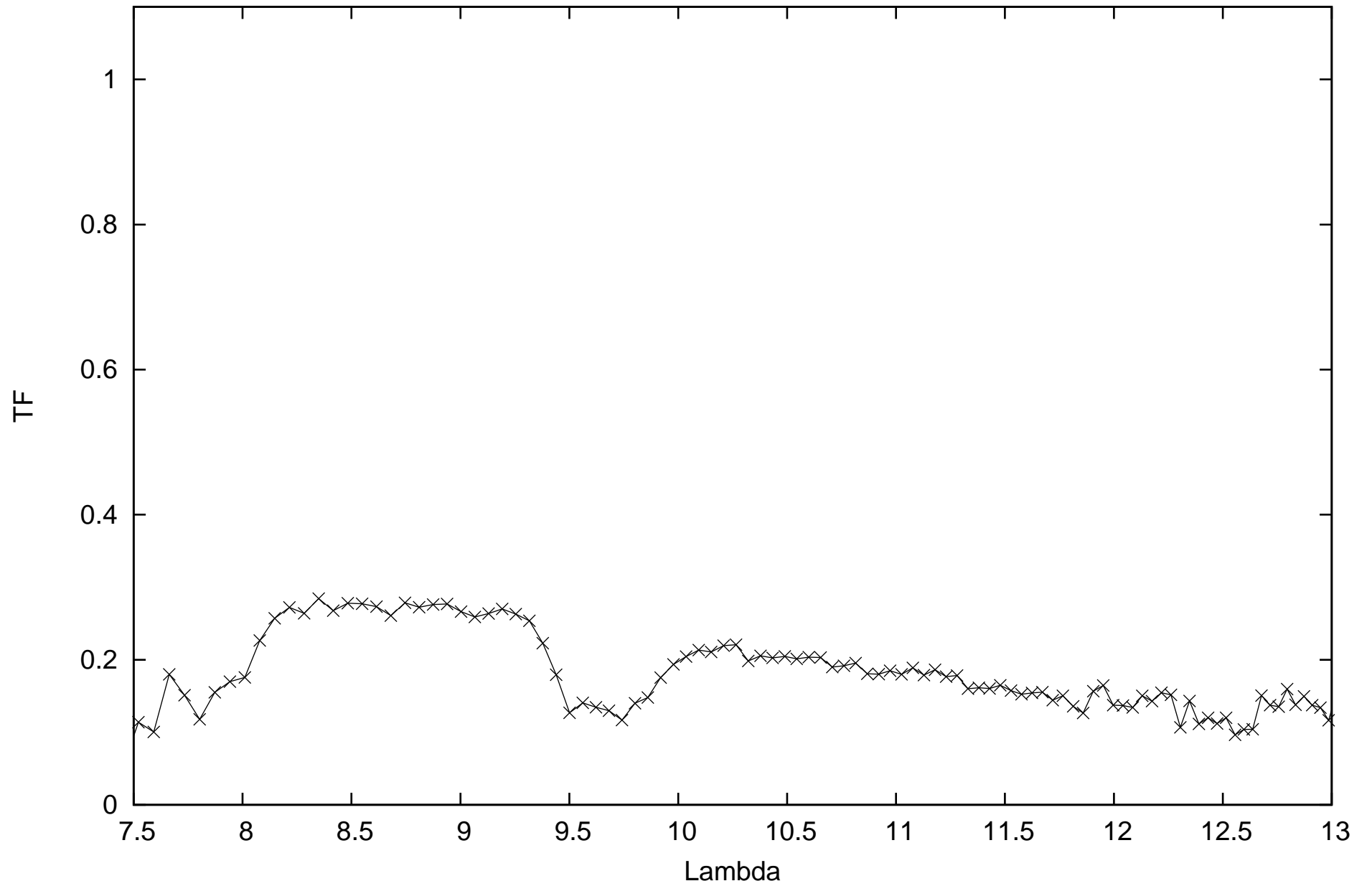
calHD107446_flux0.22_diam4.43_r.MIDI.2014-04-30T05_48_40.000_D011
