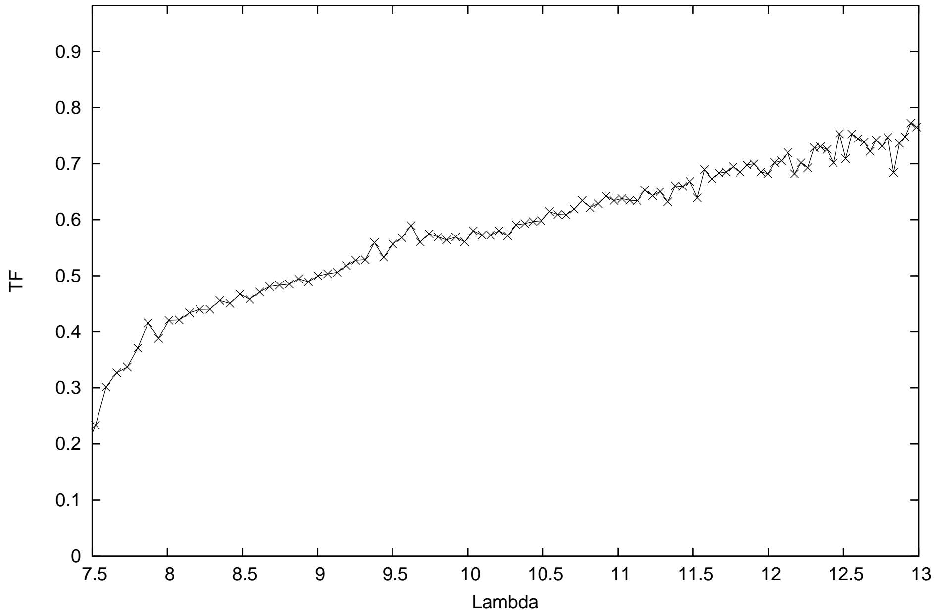
calHD81797_flux-1.49_diam9.14_r.MIDI.2014-04-11T05_07_07.000_D0G1
