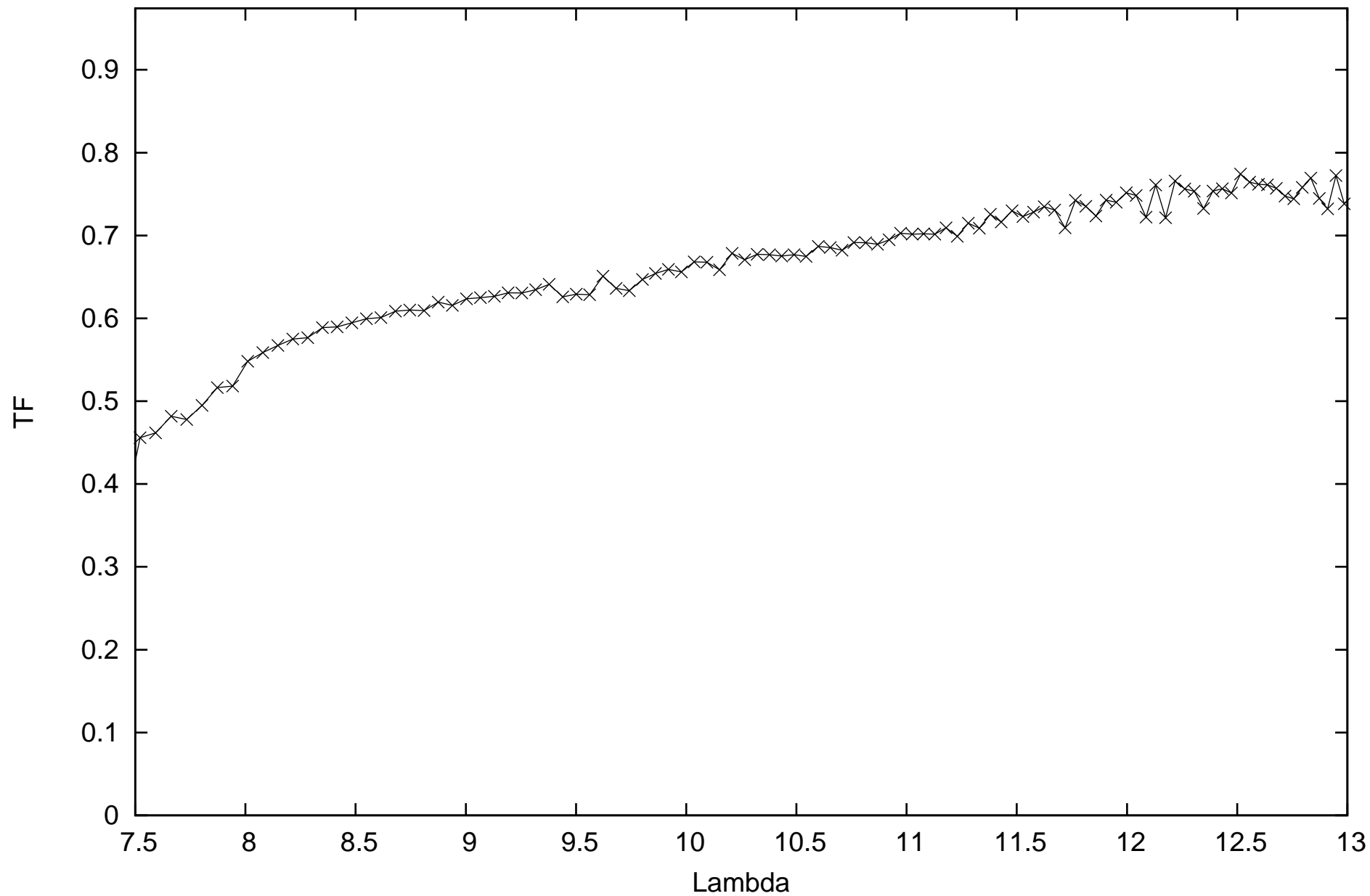
calHD81797_flux-1.49_diam9.14_r.MIDI.2014-04-11T00_32_02.000_D0G1
