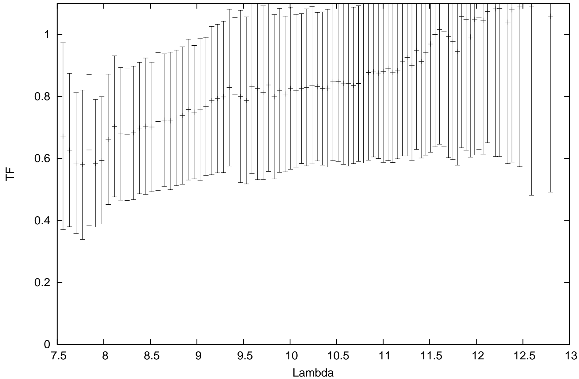
calHD81797_flux-1.49_diam9.14_r.MIDI.2014-03-27T03_28_13.113_J3K0
