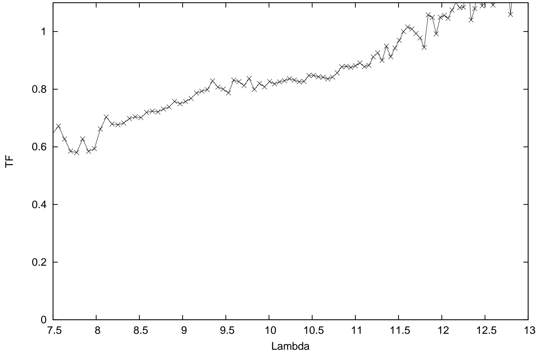
calHD81797_flux-1.49_diam9.14_r.MIDI.2014-03-27T03_28_13.113_J3K0
