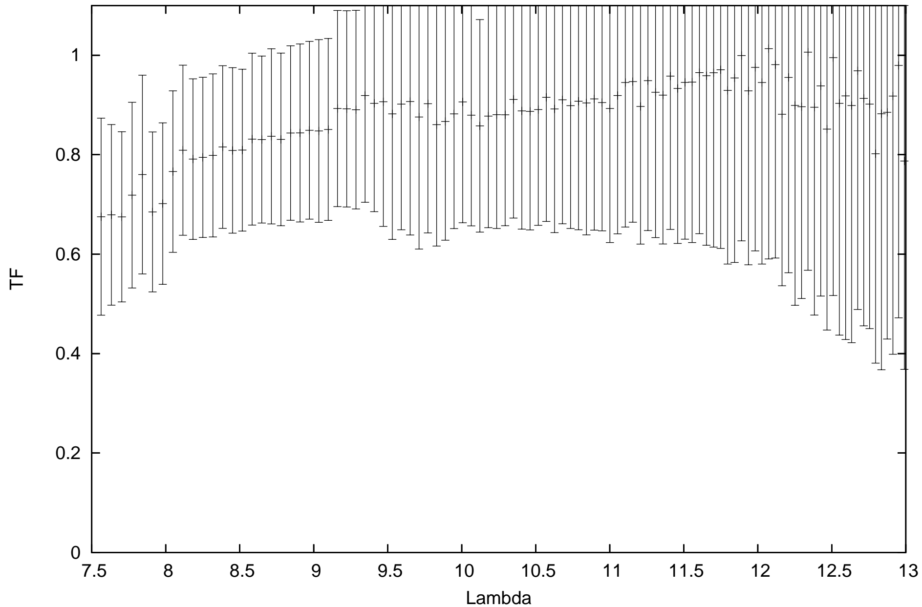
calHD48915_flux-1.39_diam6.09_r.MIDI.2014-02-11T02_55_01.135_B2A1
