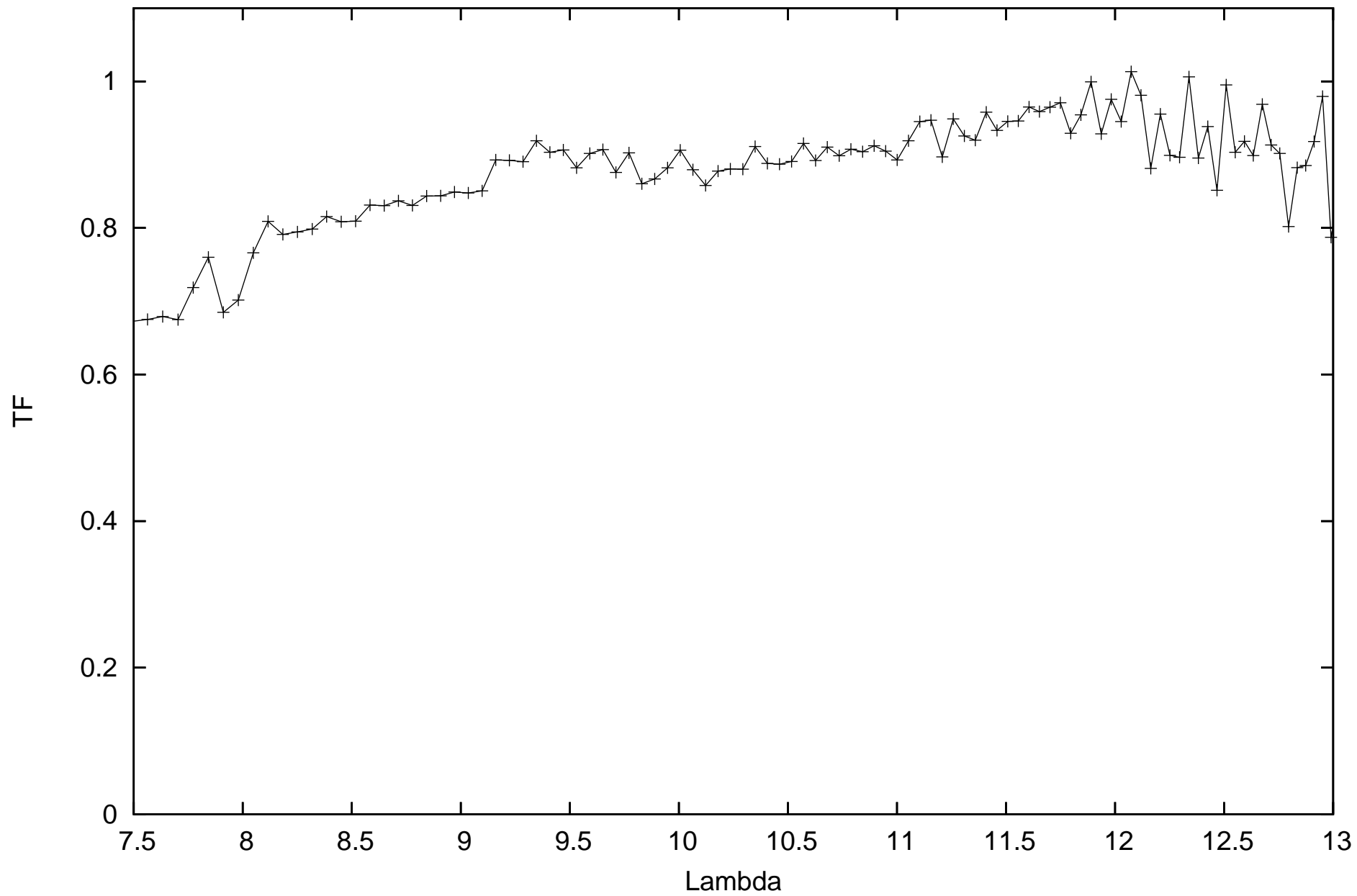
calHD48915_flux-1.39_diam6.09_r.MIDI.2014-02-11T02_55_01.135_B2A1
