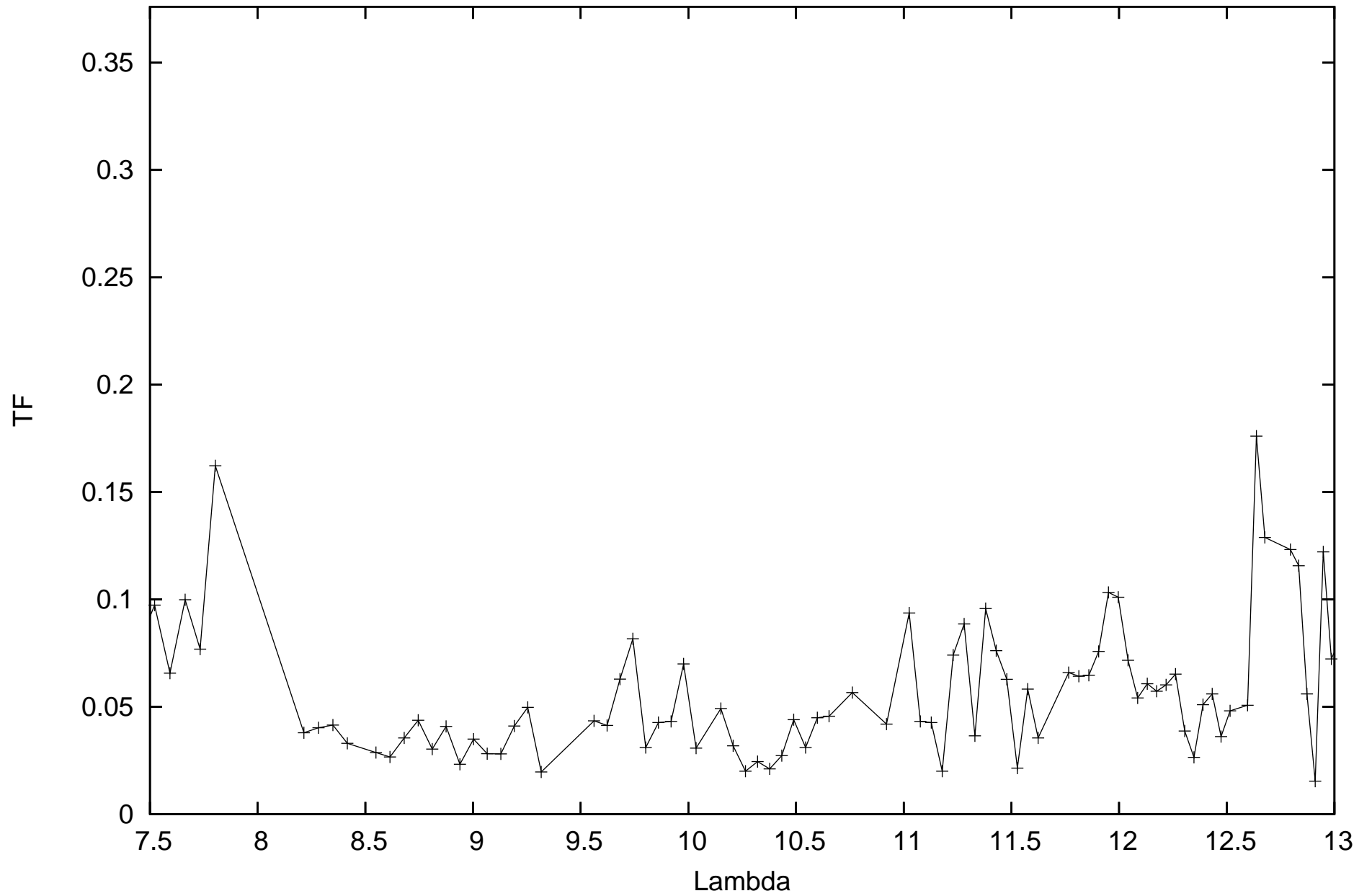
calHIP57512_flux1.13963_diam2.98_r.MIDI.2014-02-07T03_17_54.000_D0H0
