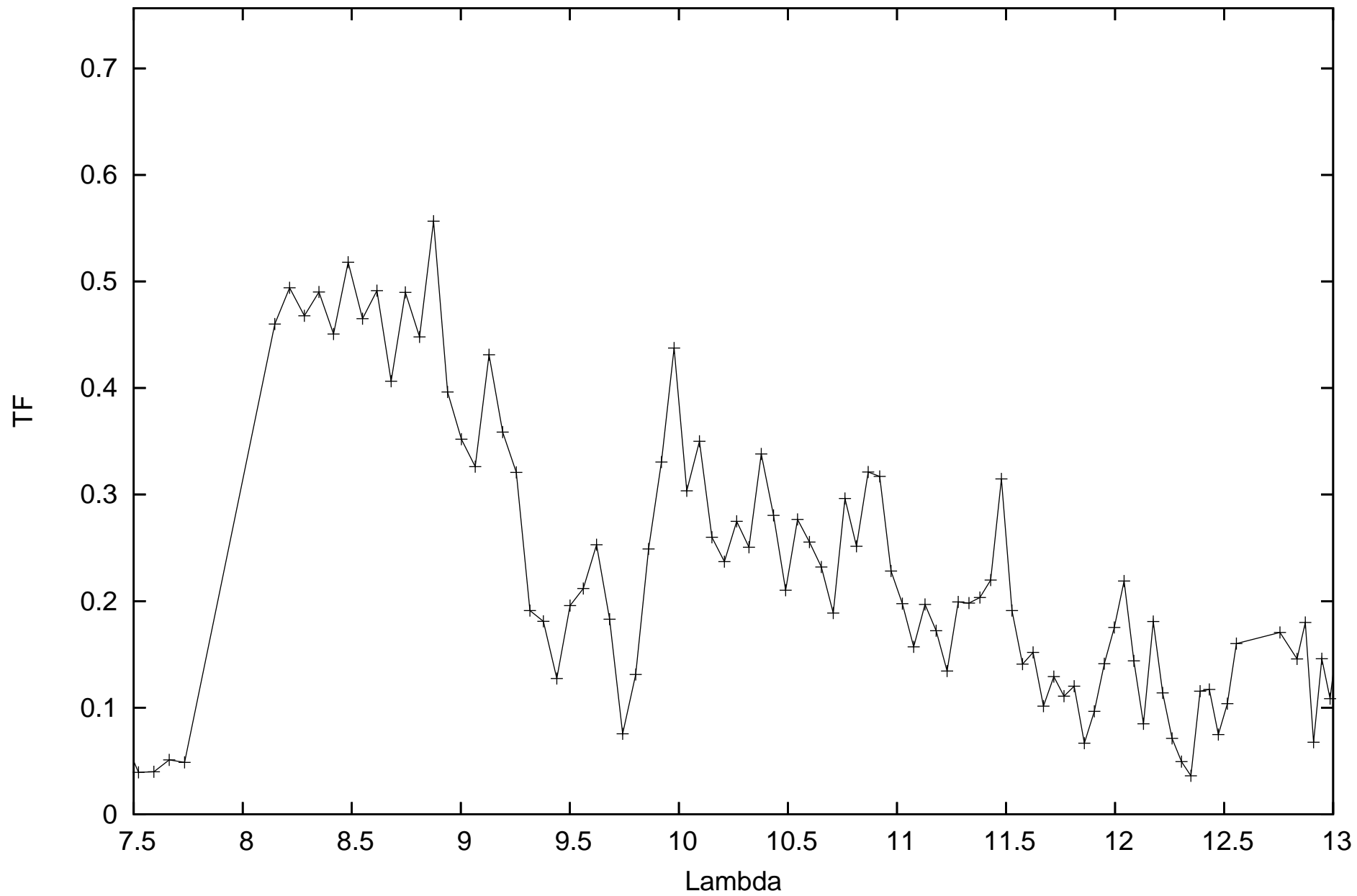
calHD98292_flux0.92_diam3.35_r.MIDI.2014-02-07T04_27_23.000_H0G1
