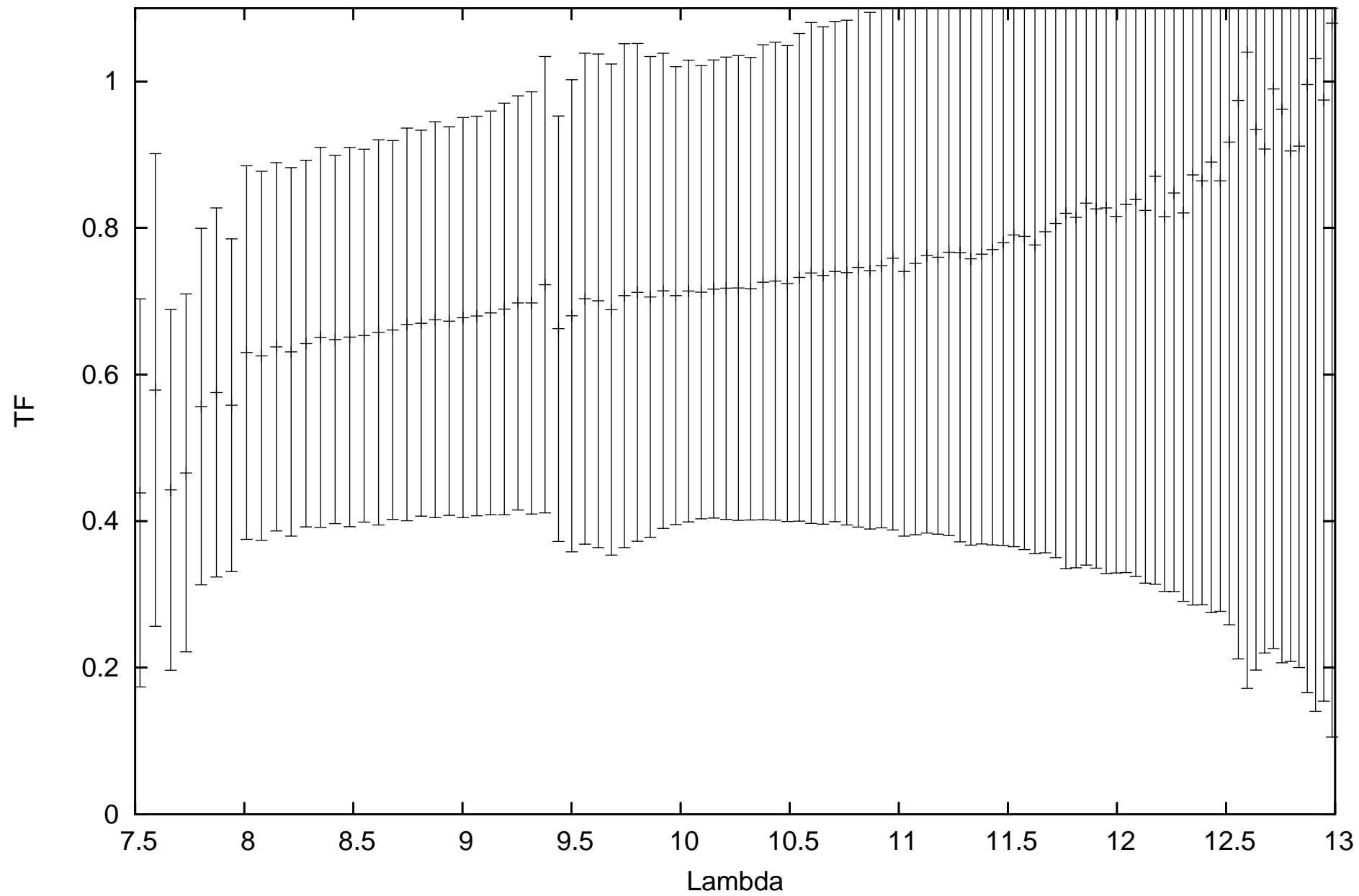
calHIP15549_flux0.657635_diam3.64_r.MIDI.2014-01-15T02_43_46.000_U2U4
