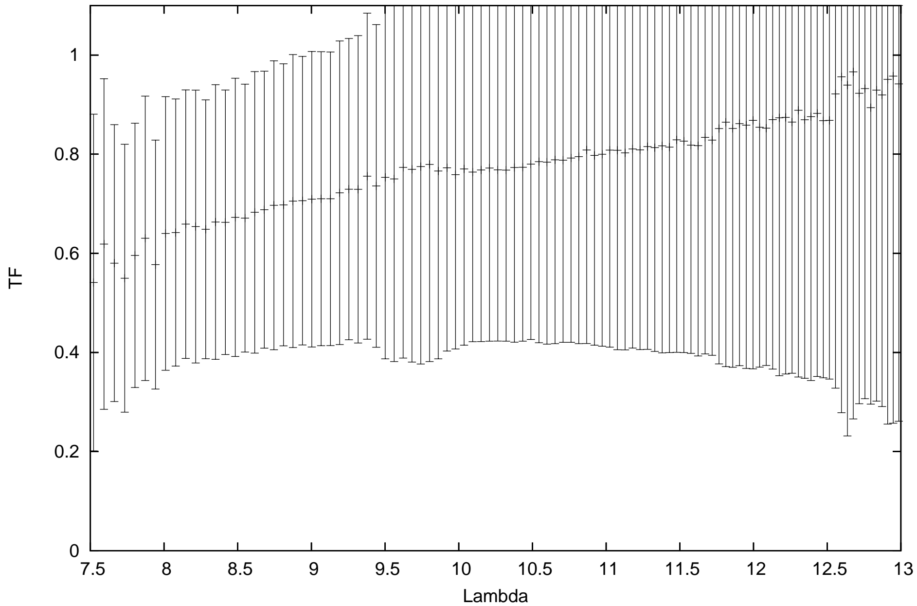
calHIP15549_flux0.657635_diam3.64_r.MIDI.2014-01-15T00_42_57.000_U2U4
