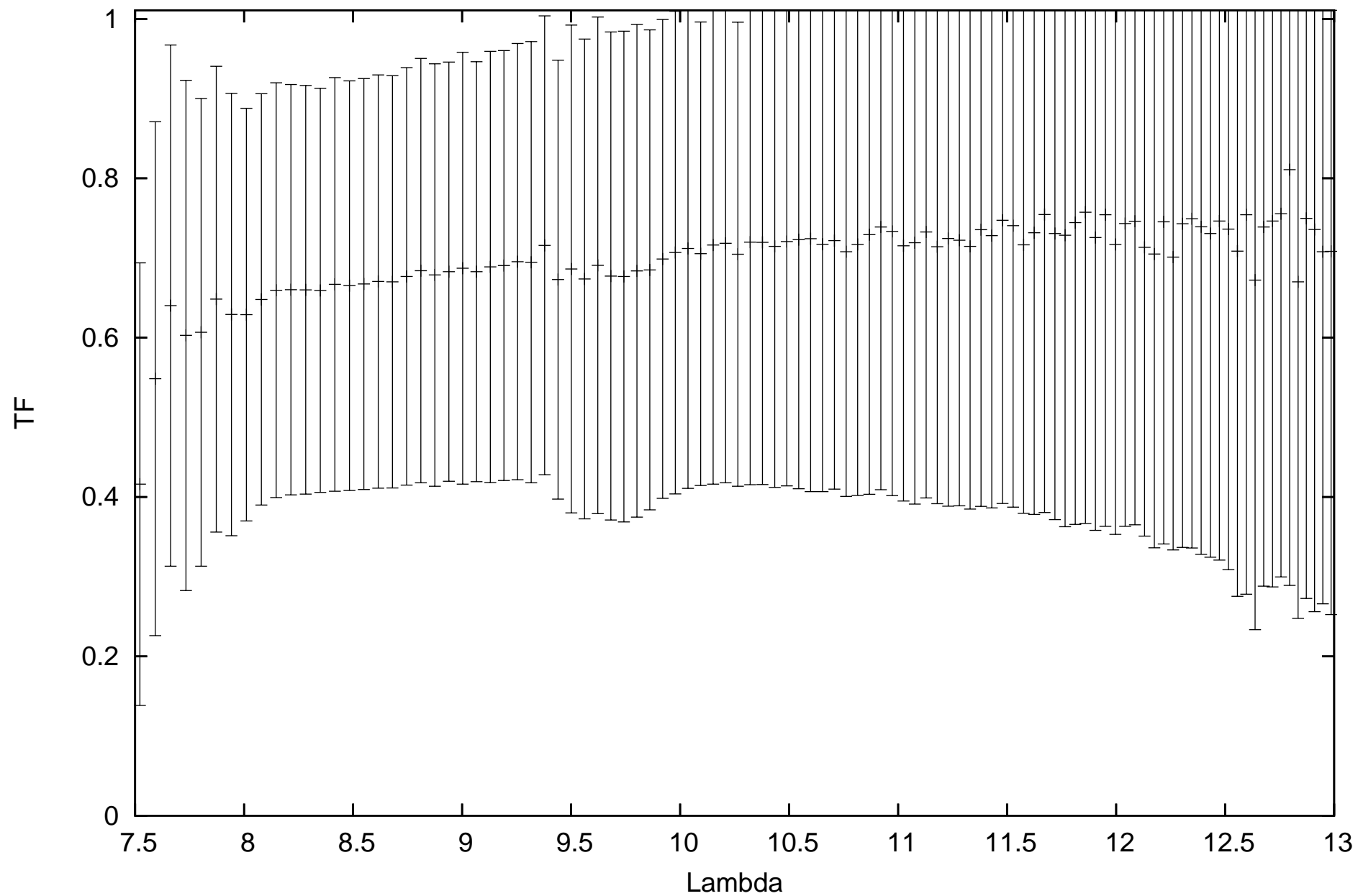
calHIP19038_flux1.83316_diam1.9_r.MIDI.2014-01-14T02_27_00.000_U1U3
