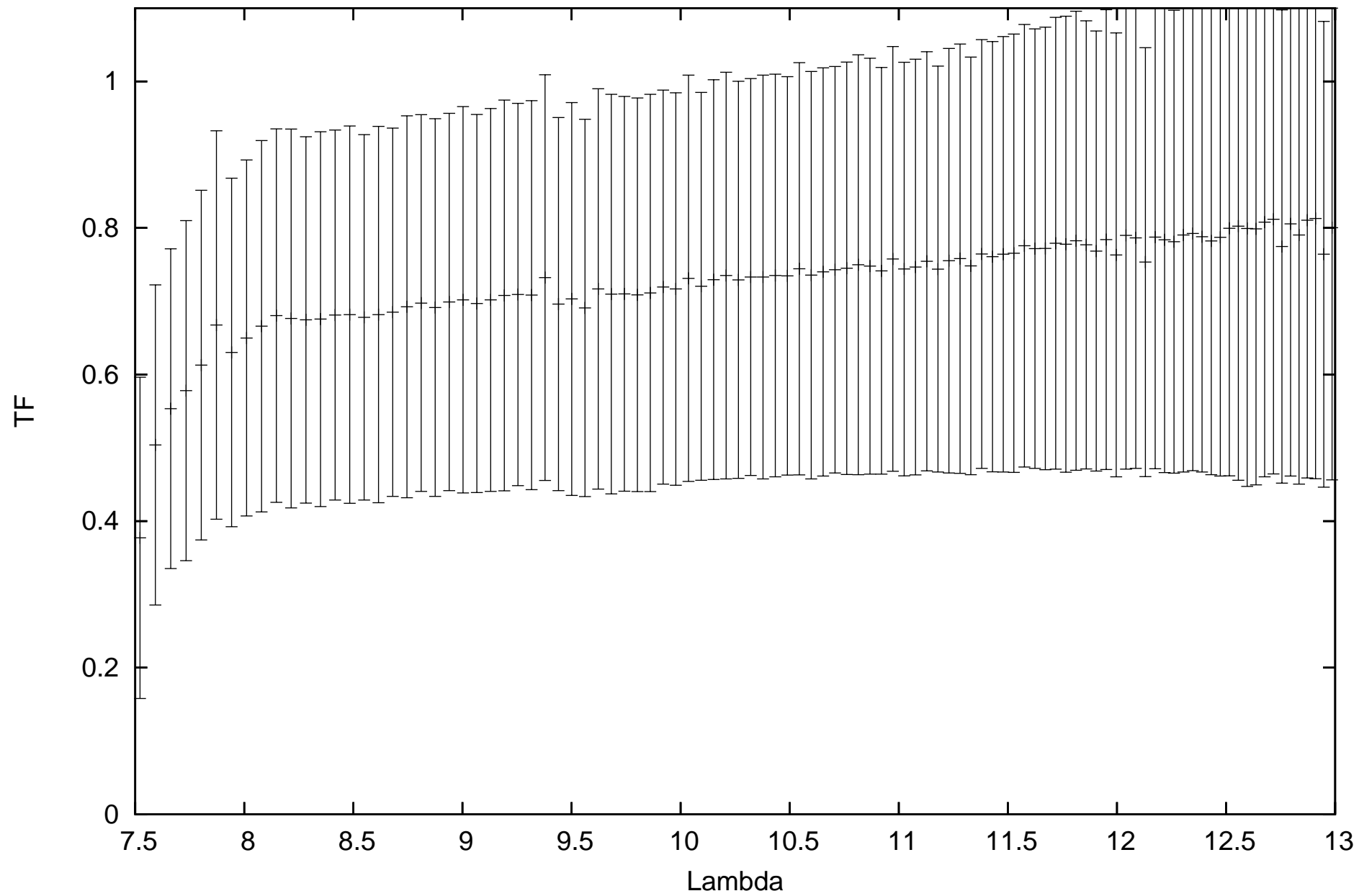
calHIP15549_flux0.657635_diam3.64_r.MIDI.2014-01-14T01_17_39.000_U1U3
