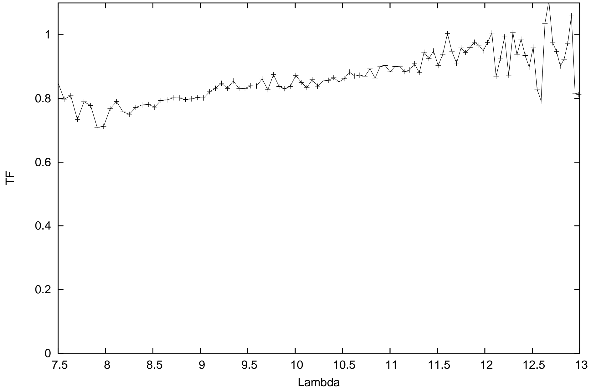
calHD81797_flux-1.49_diam9.14_r.MIDI.2014-01-11T08_53_23.970_C1B2
