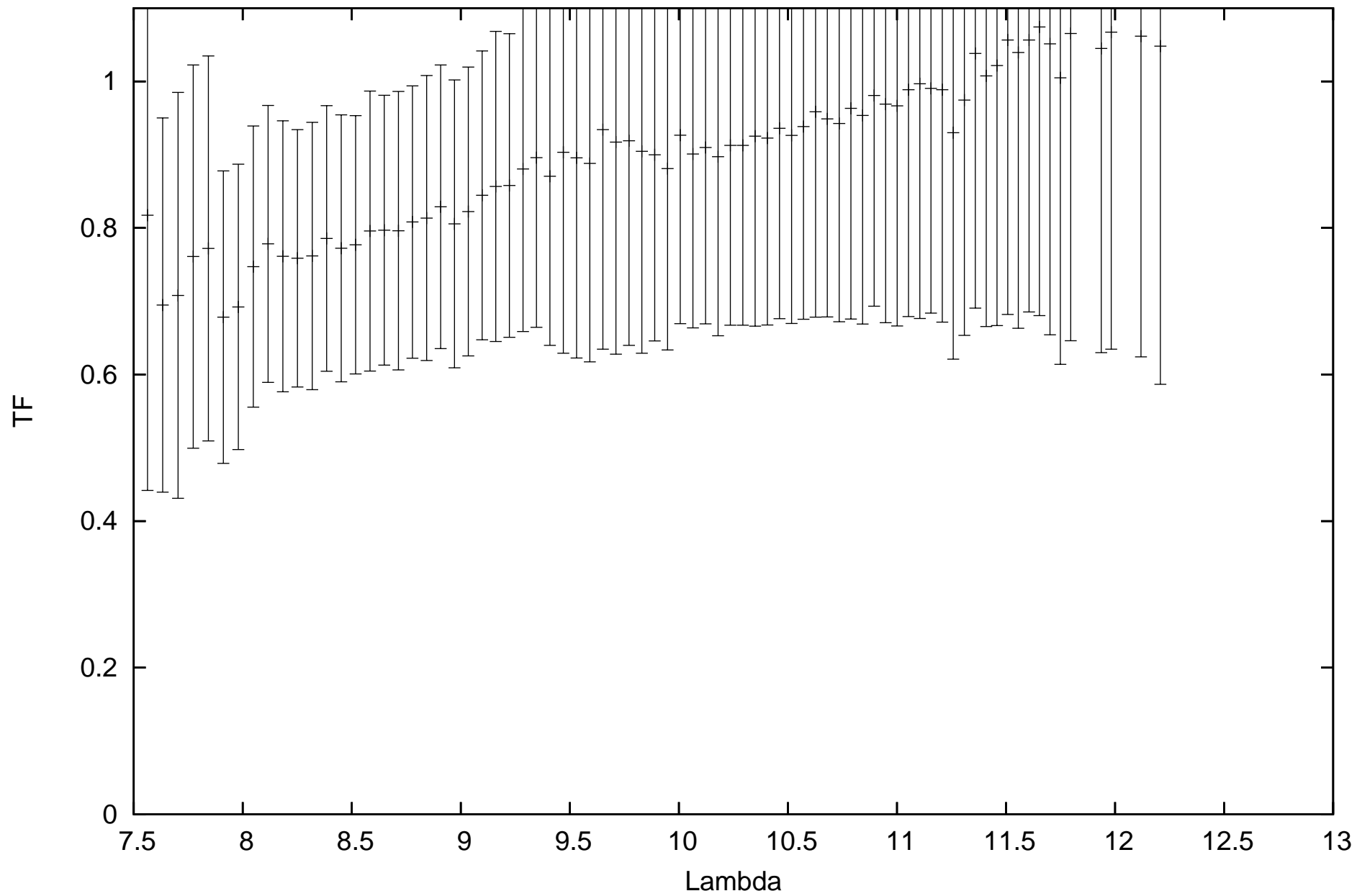
calHD81797_flux-1.49_diam9.14_r.MIDI.2014-01-11T08_15_45.135_D0C1
