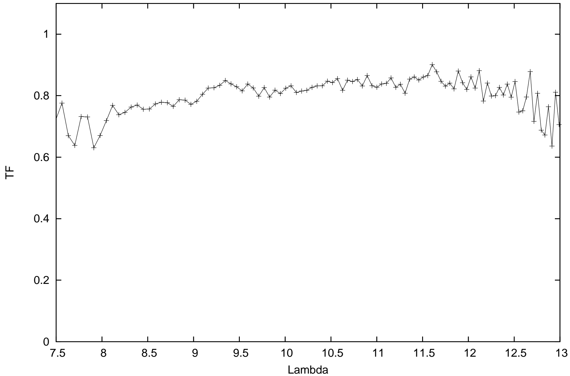
calHD81797_flux-1.49_diam9.14_r.MIDI.2014-01-11T07_01_10.135_B2A1
