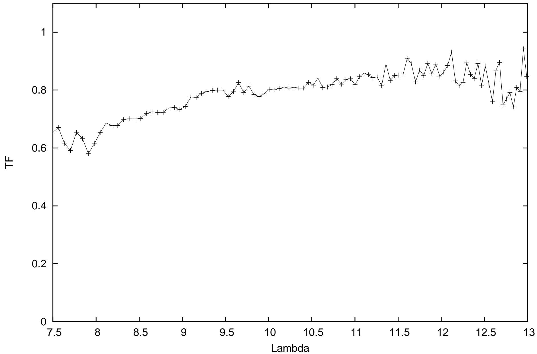
calHD81797_flux-1.49_diam9.14_r.MIDI.2014-01-11T05_48_47.970_C1A1
