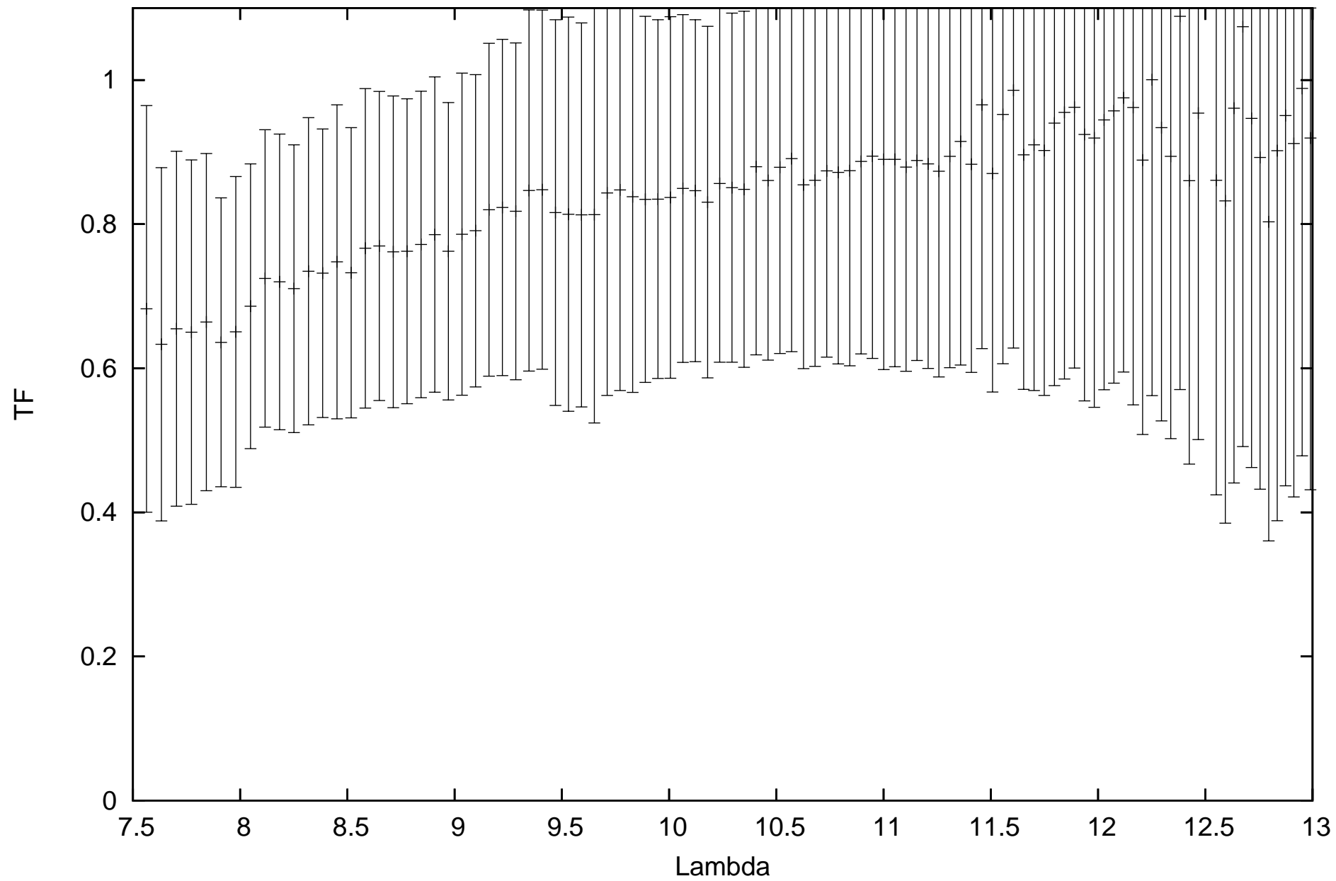
calHD81797_flux-1.49_diam9.14_r.MIDI.2014-01-11T04_35_05.970_D0C1
