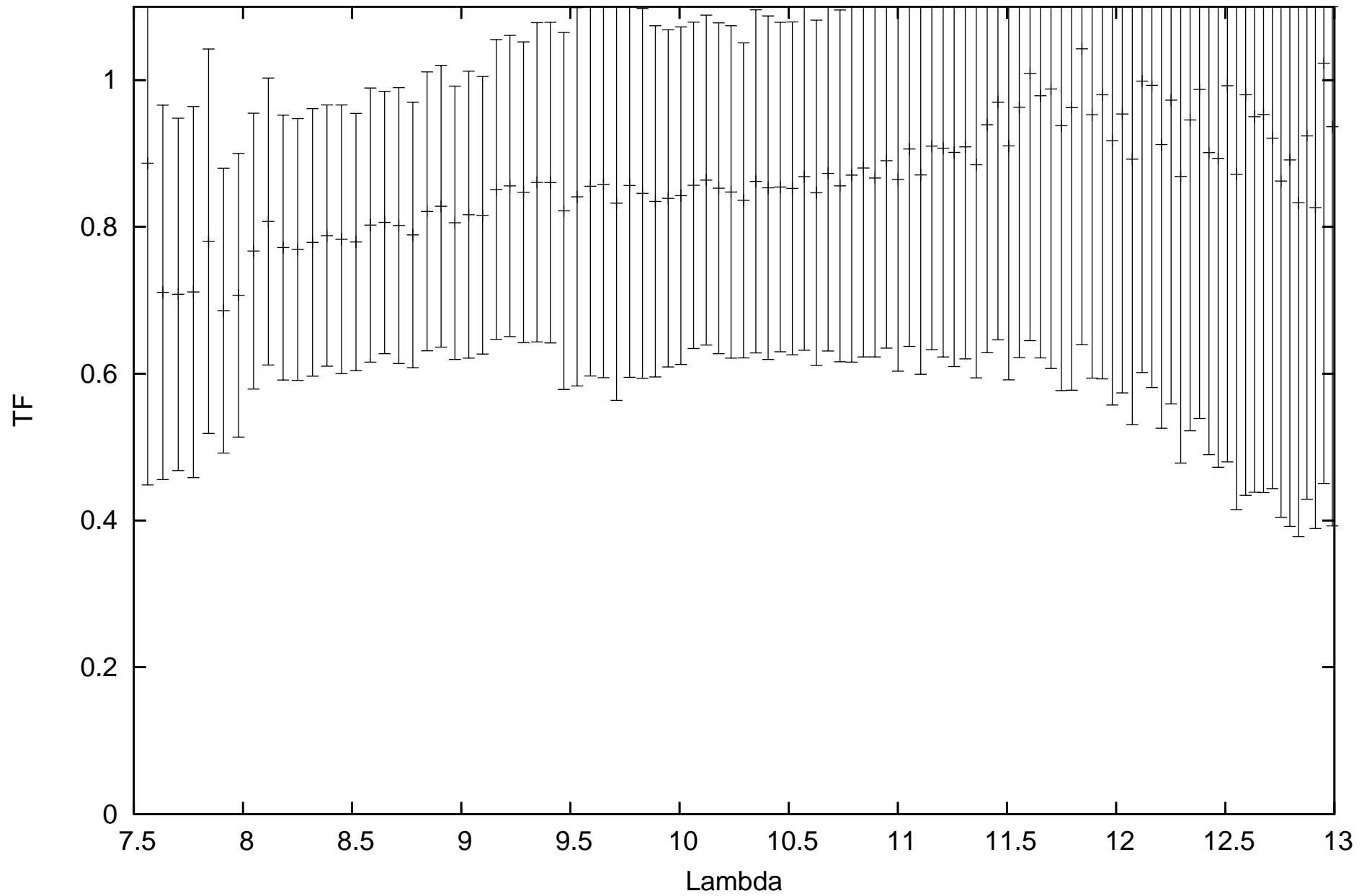
calHD48915_flux-1.39_diam6.09_r.MIDI.2014-01-10T06_34_42.932_C1A1
