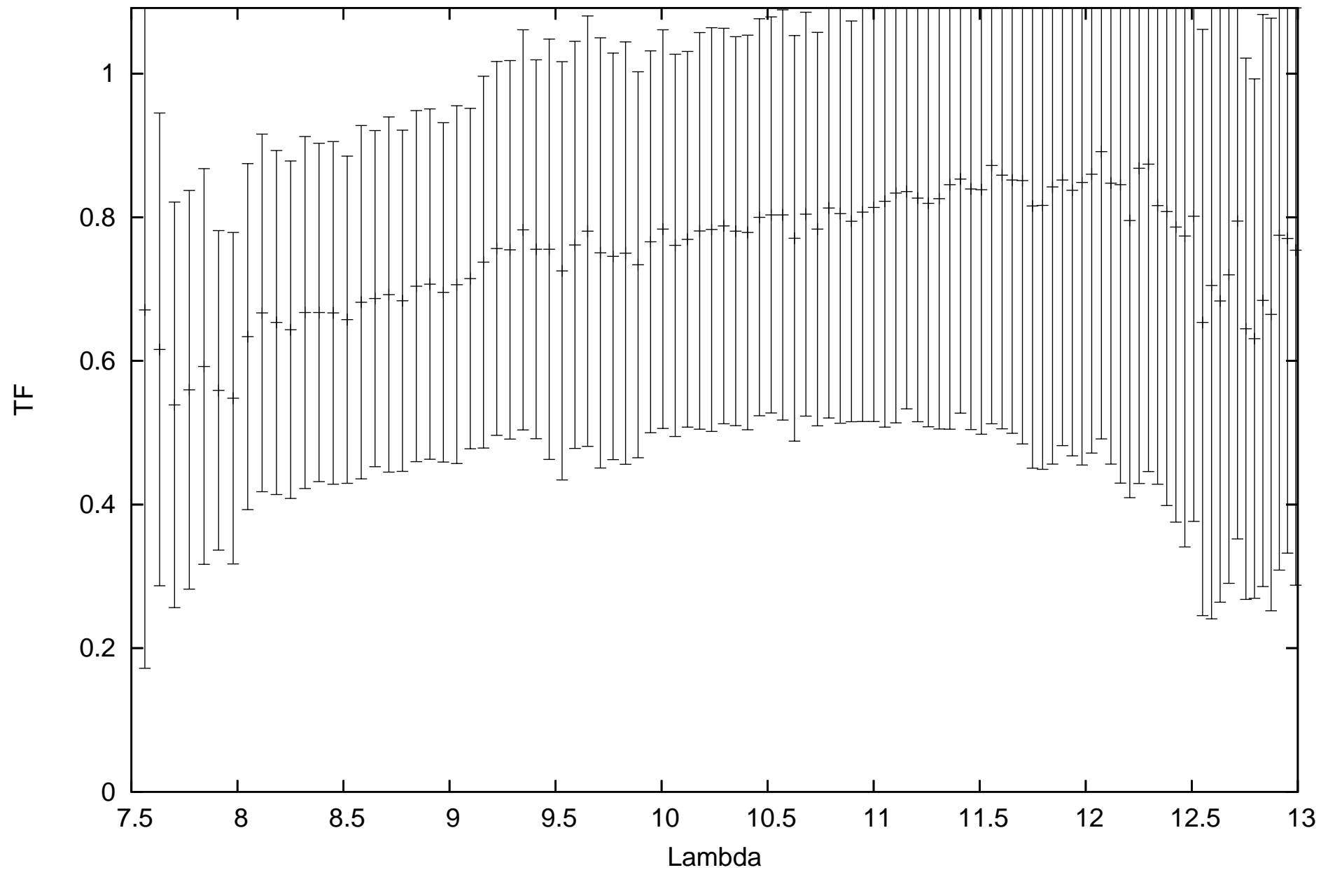
calHD81797_flux-1.49_diam9.14_r.MIDI.2014-01-09T07_06_23.113_B2A1
