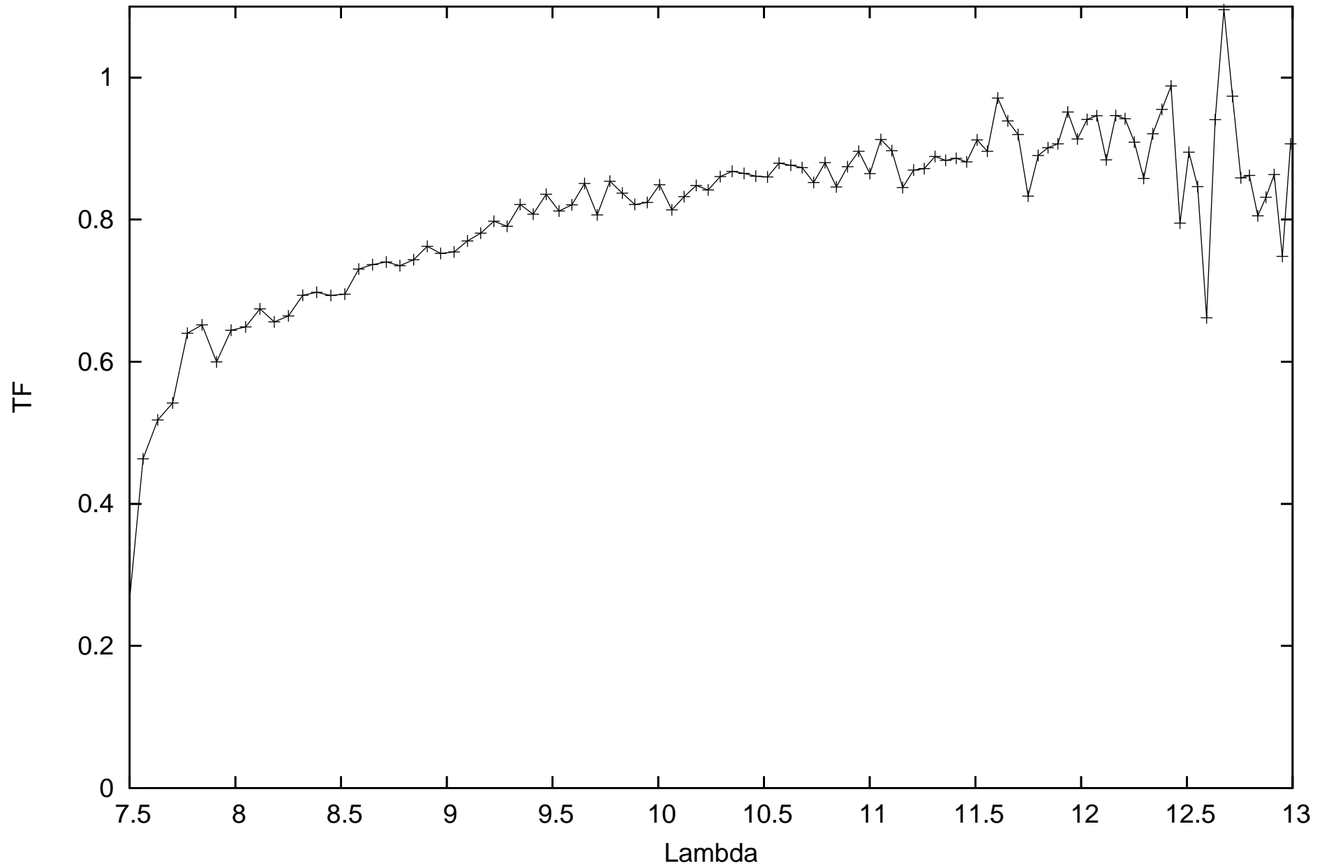
calHD48915_flux-1.39_diam6.09_r.MIDI.2014-01-06T05_54_59.970_D0H0
