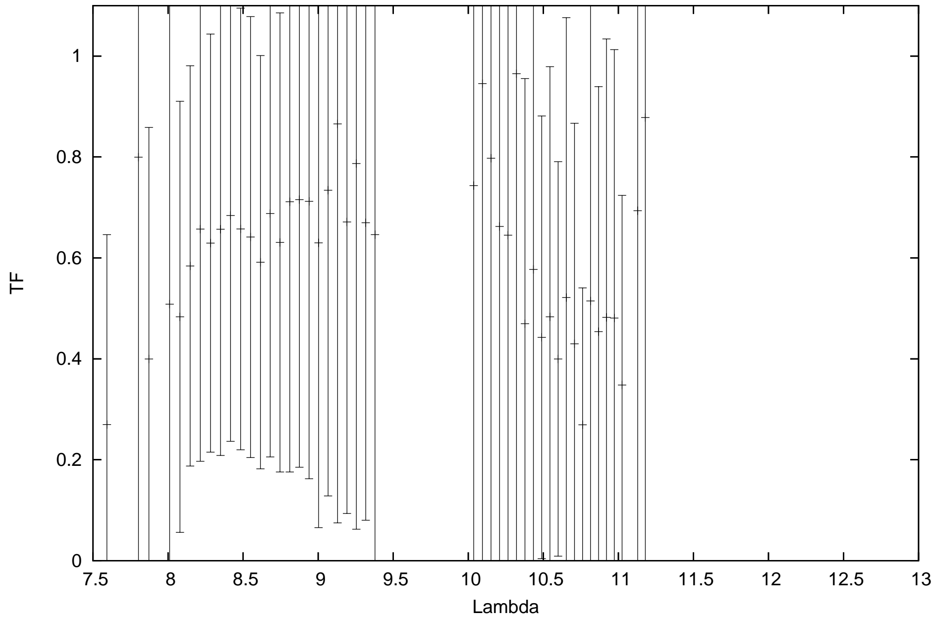
calHD44033_flux1.56_diam2.48_r.MIDI.2014-01-06T04_01_51.000_G111
